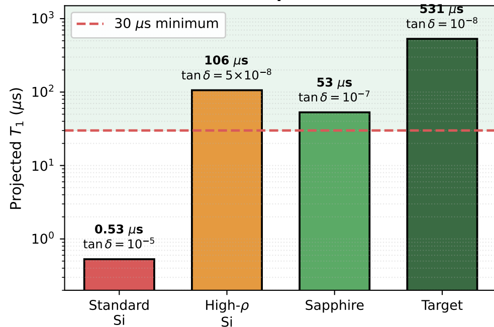
(b) Substrate comparison at 300 GHz
