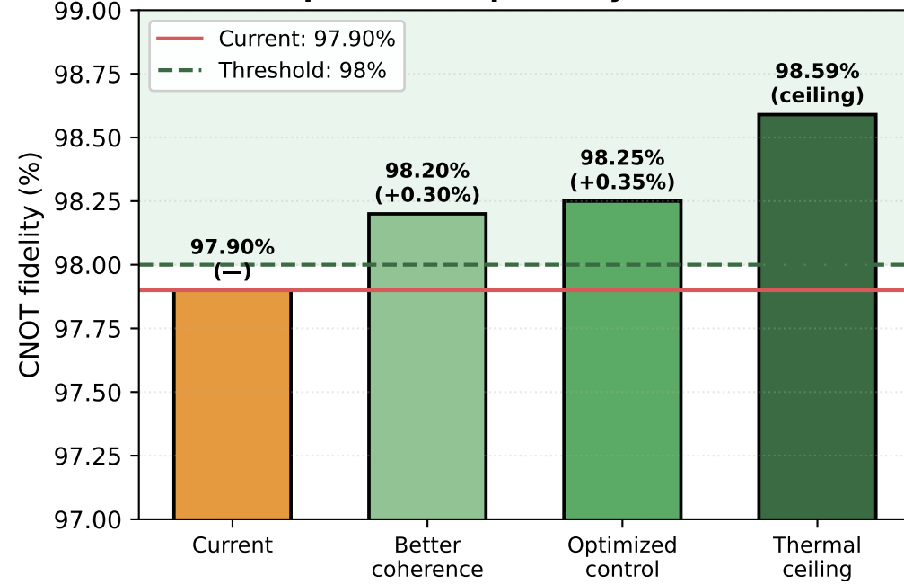
(c) Improvement pathways at fixed 4 K
