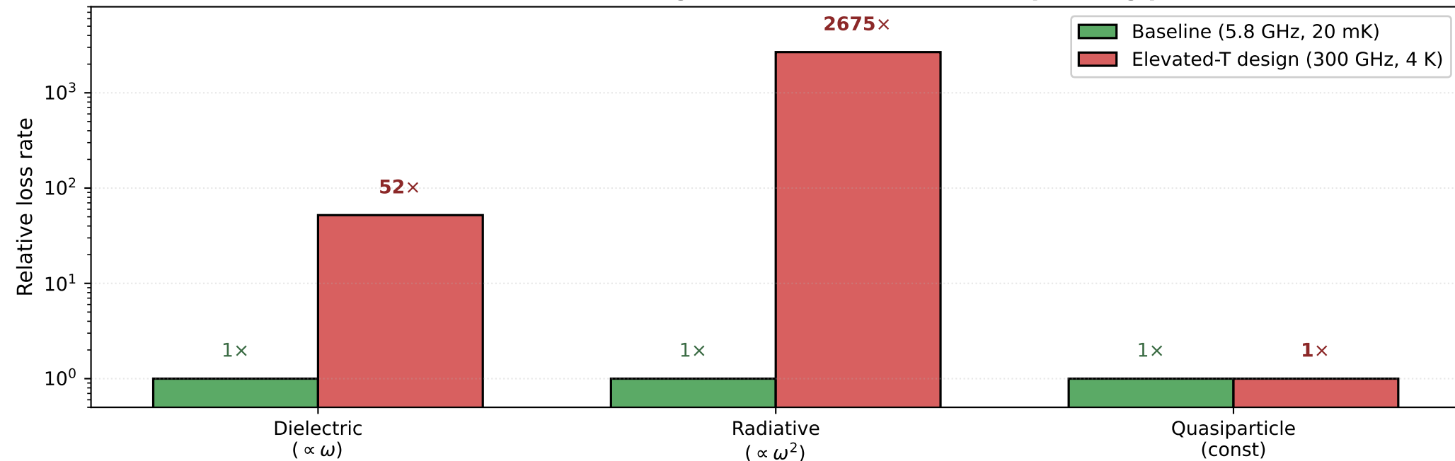
(a) Loss-mechanism scaling: baseline vs. elevated-T operating point
