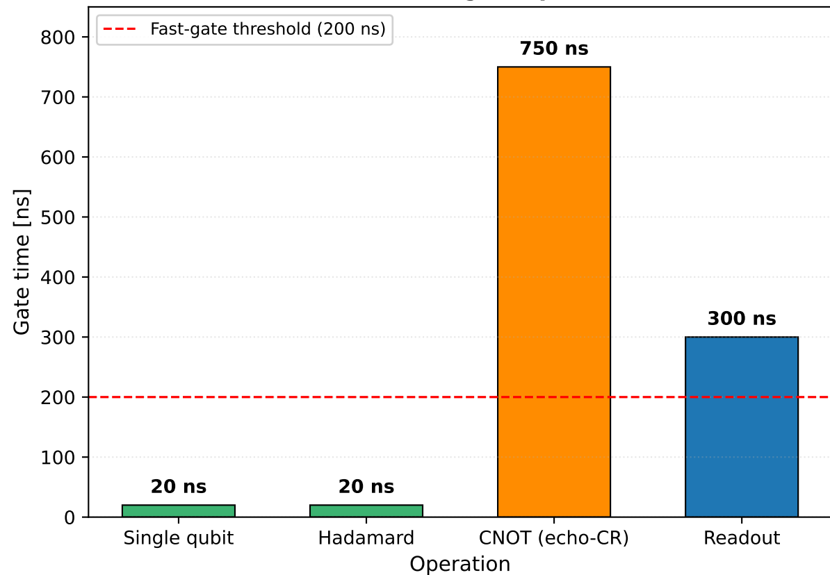
(b) Gate timing comparison
