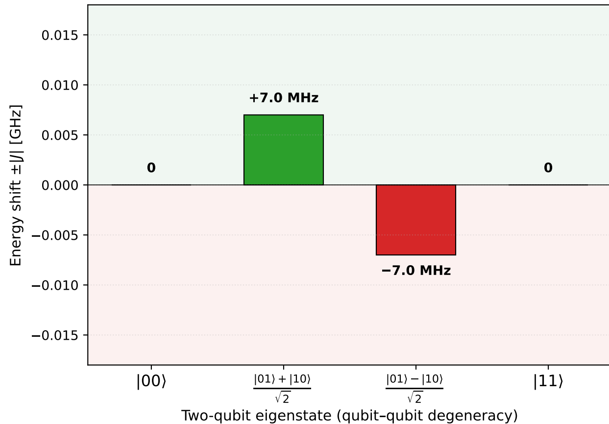
(a) Cavity-mediated transverse exchange |J|/2\pi = 7.0 MHz
