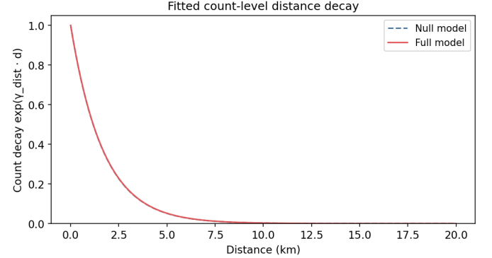
Fig. 3. Fitted distance-decay factor \exp(\hat{\gamma}_{\text{dist}} \cdot d) vs. haversine distance. Demand decays approximately 50% per km.
