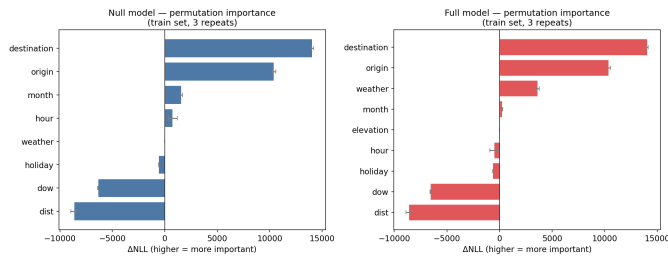
Fig. 4. Permutation feature importance ( \Delta\text{NLL} , 3 repeats). Station fixed effects dominate; weather contributes meaningfully; elevation is marginal.
