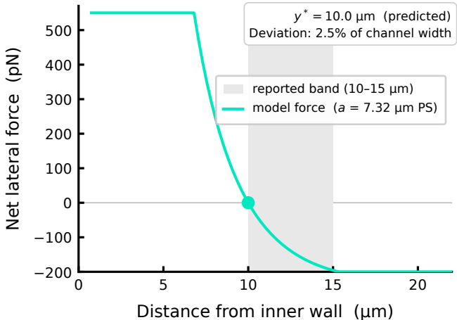
Bhagat (2008) validation, 7.32 \mu\text{m} polystyrene beads
