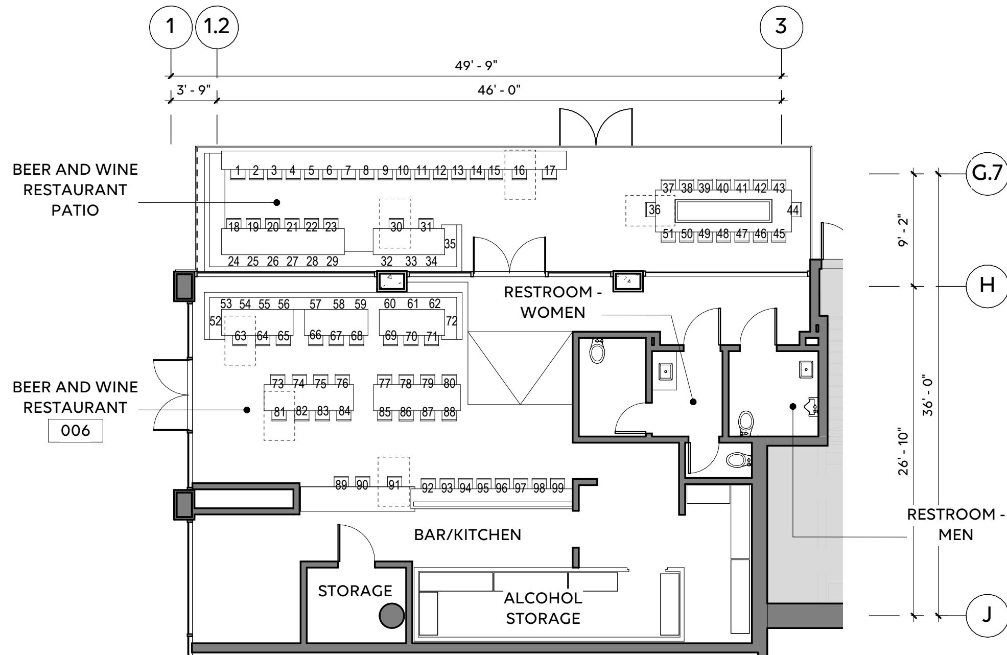
BEER AND WINE RESTAURNT - 006 1/8" = 1'-0"
