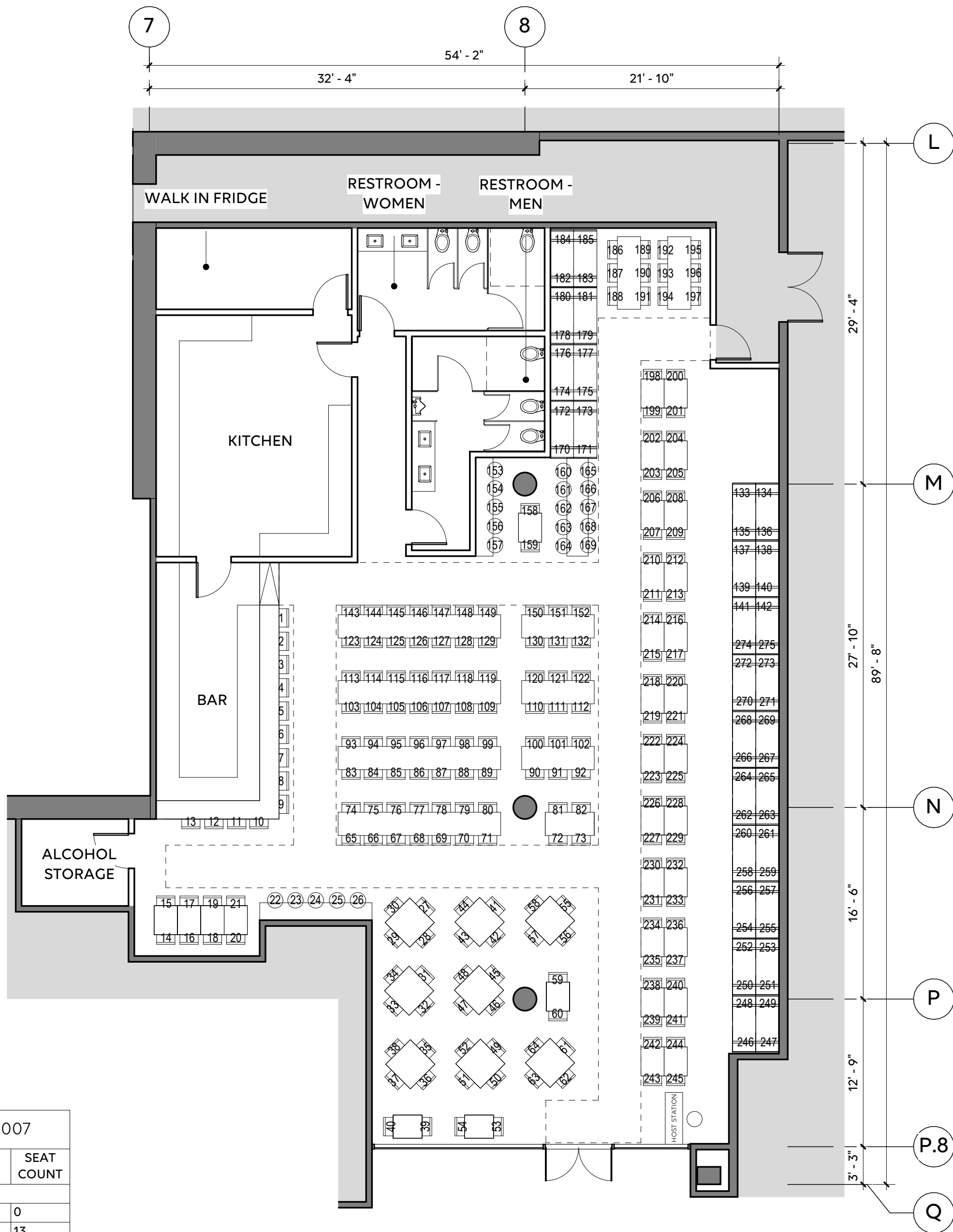
BEER AND WINE RESTAURANT- 007 1/8" = 1'-0"
