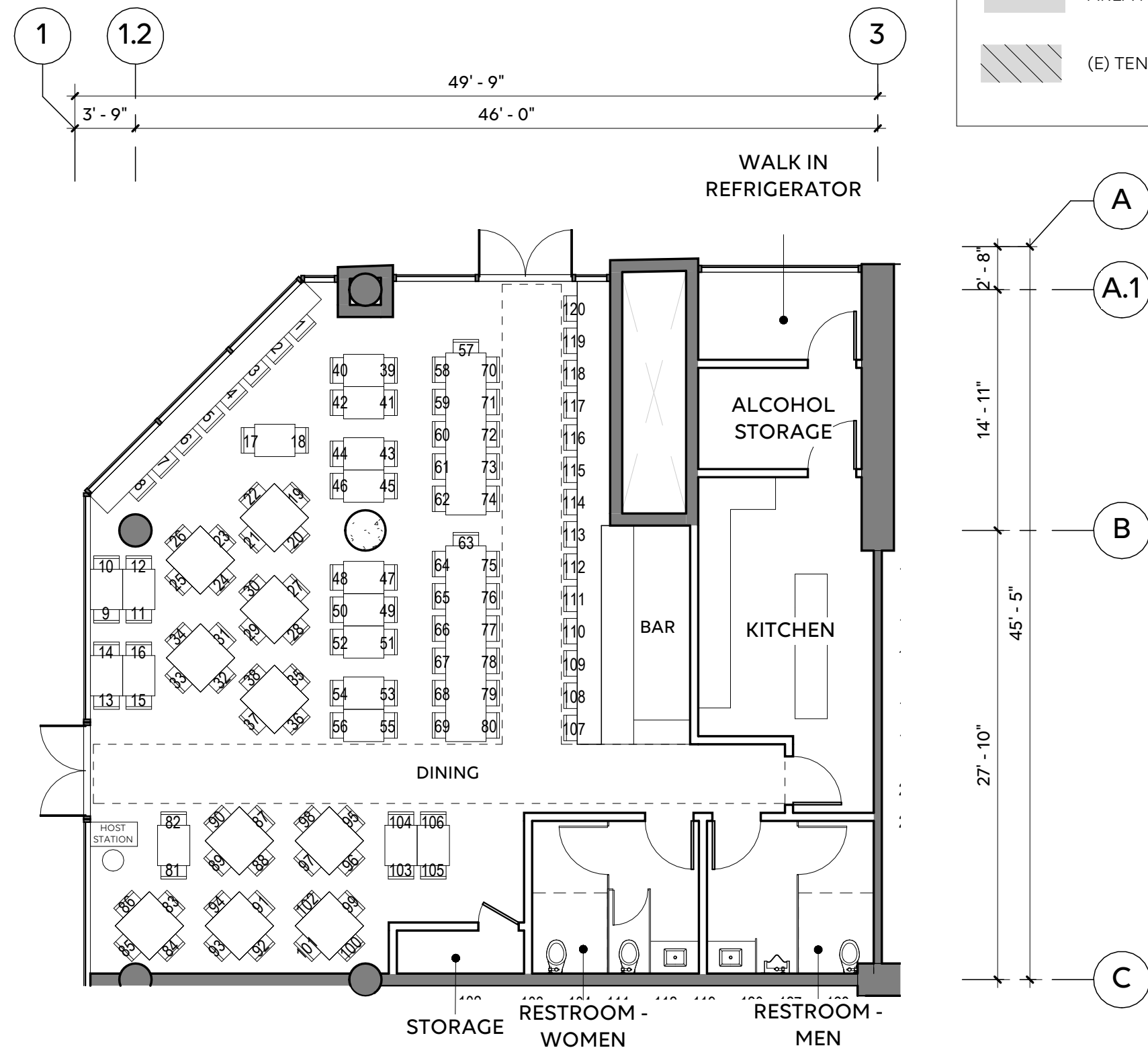
BEER AND WINE RESTAURANT - 002
