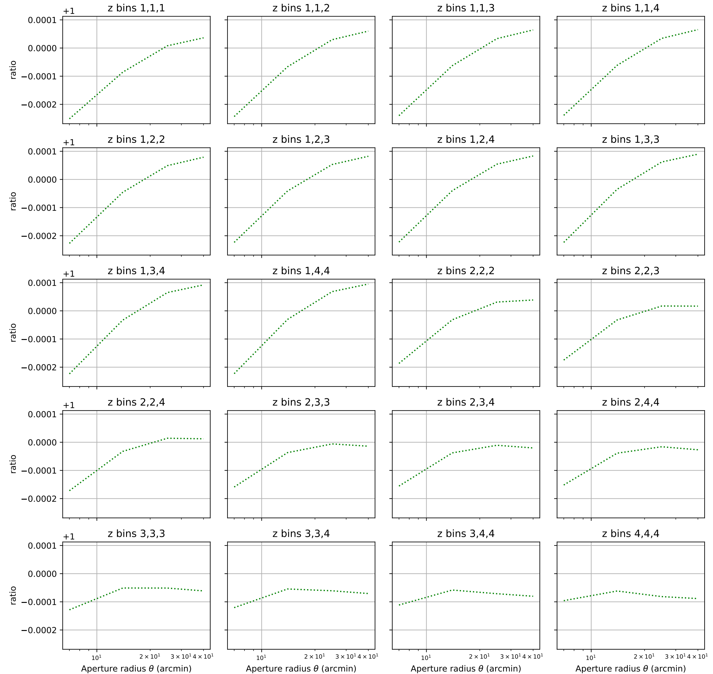
\langle M_{ap}^3 \rangle emulator/theory ratio with same z bin scheme
