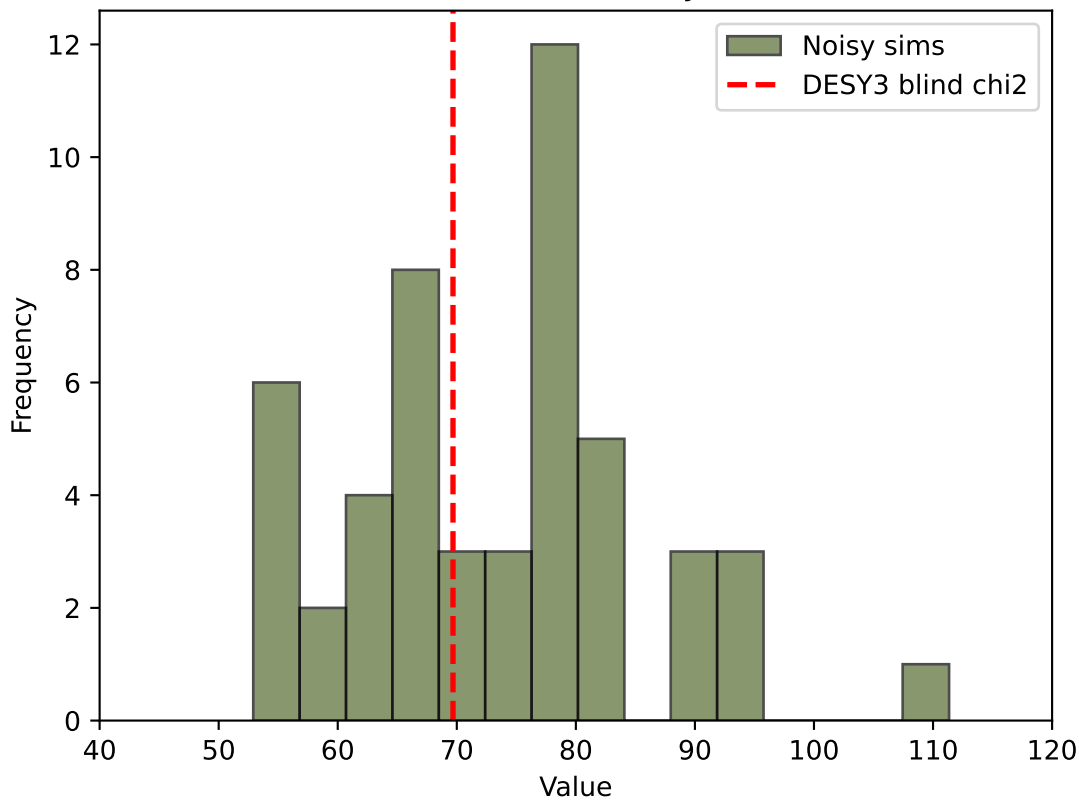
Chi2 values for noisy sims
