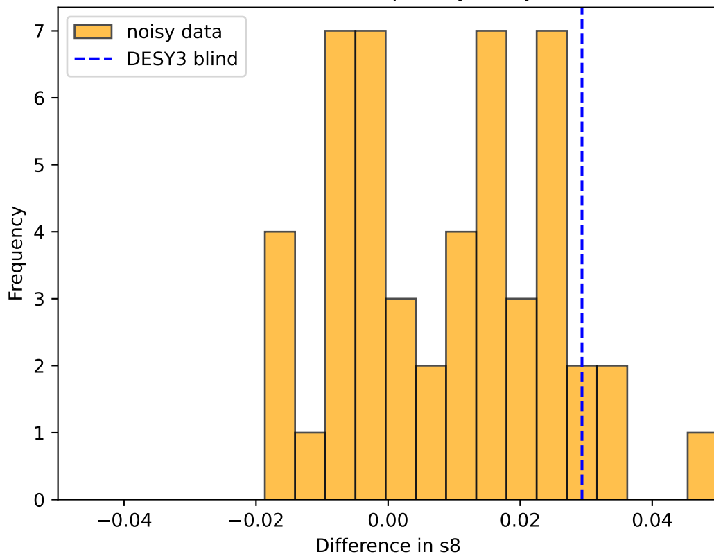
s8 difference between 2pt-only and joint chains
