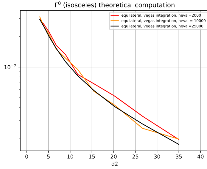
Figure 5. Isosceles \Gamma^0 shear 3pt function for a fiducial cosmology, with different number of evaluations. In all cases, 5 iterations were taken. Computation time is approximately 0.005 seconds per d_2 value per evaluation.
