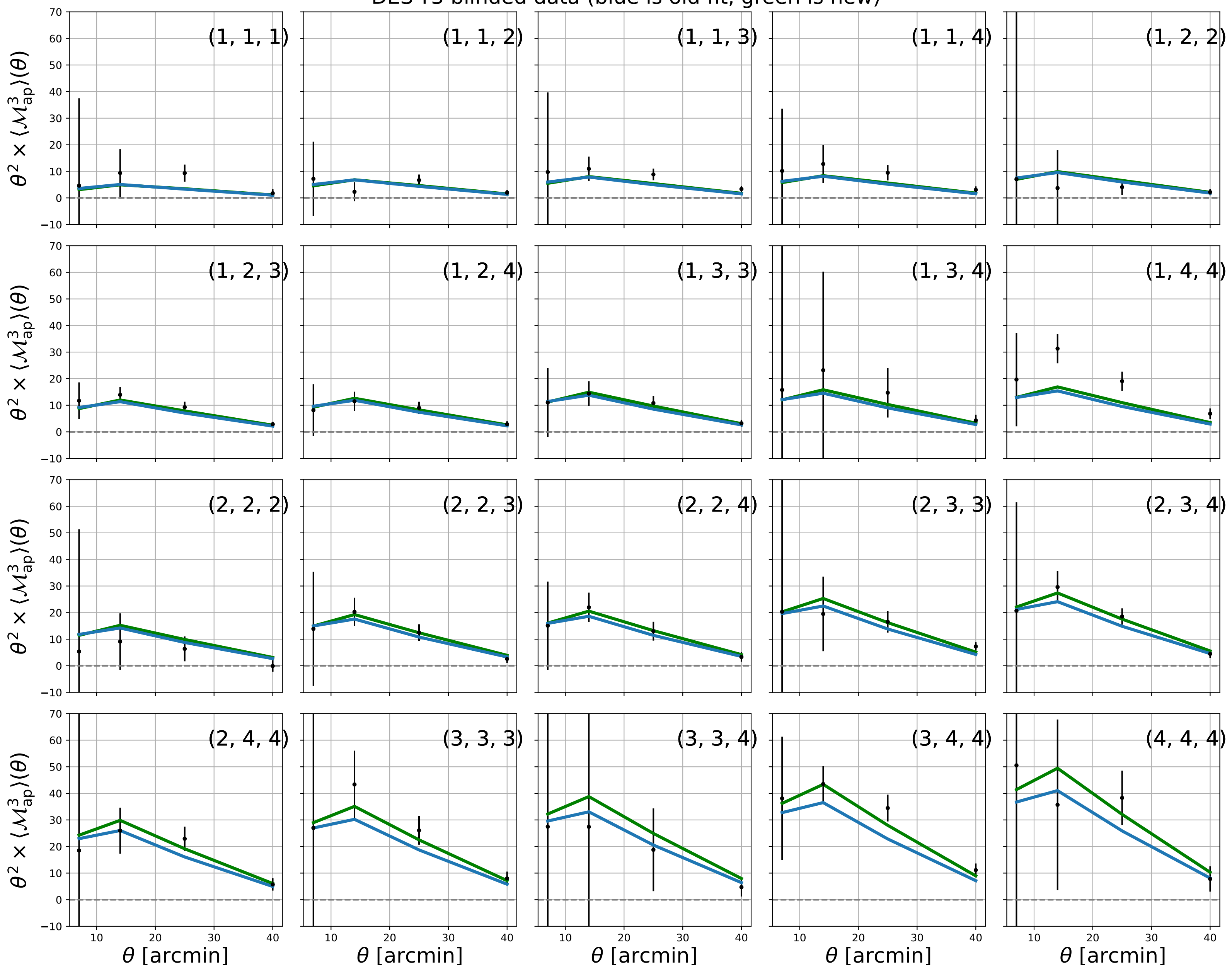
DES-Y3 blinded data (blue is old fit, green is new)
