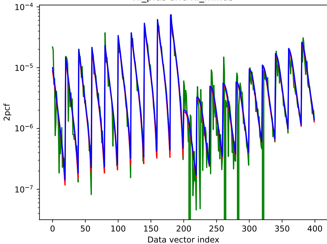
xi_plus and xi_minus
