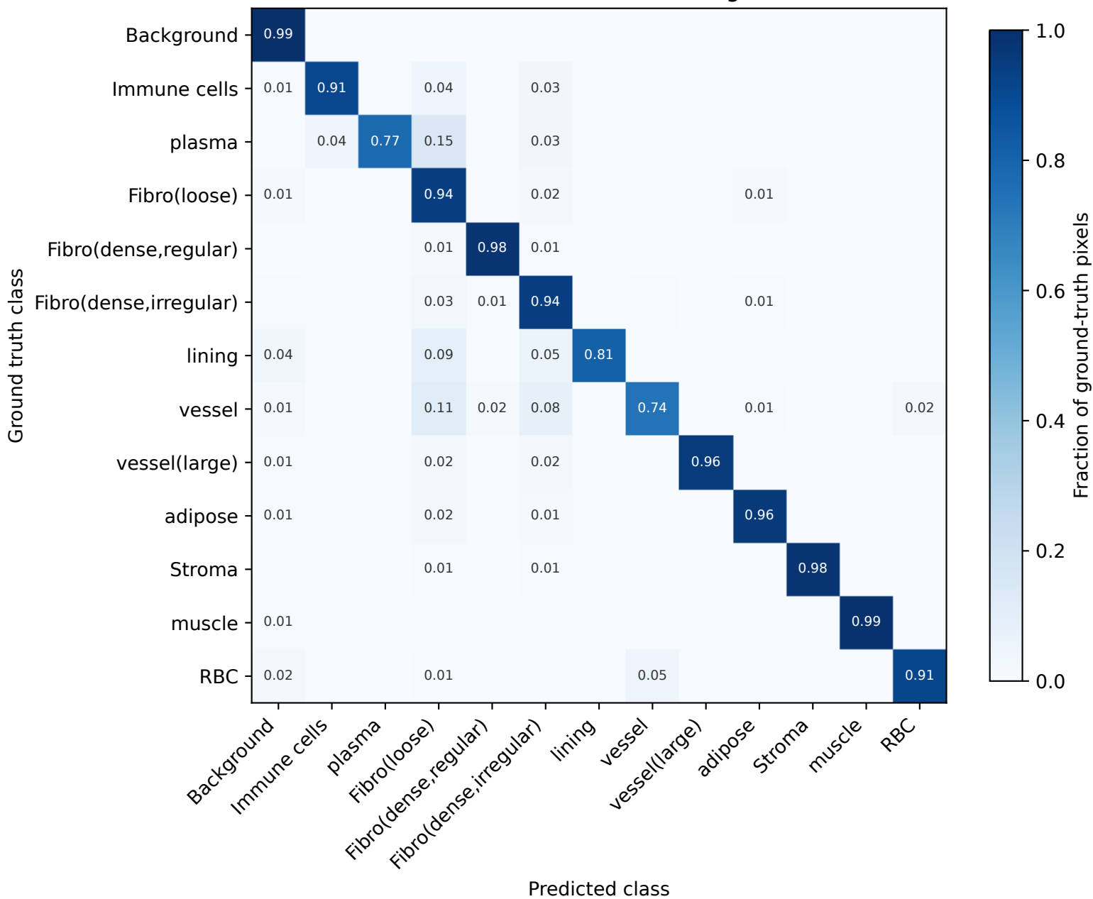
Confusion matrix (row-normalized, training set)
