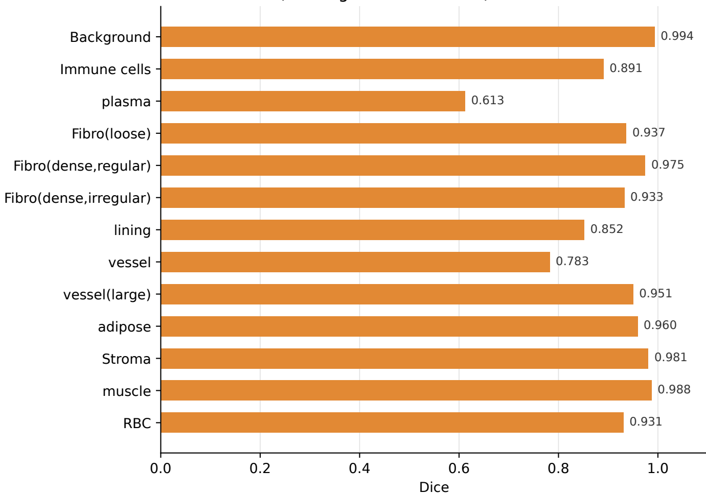
Per-class Dice (training + validation set)
