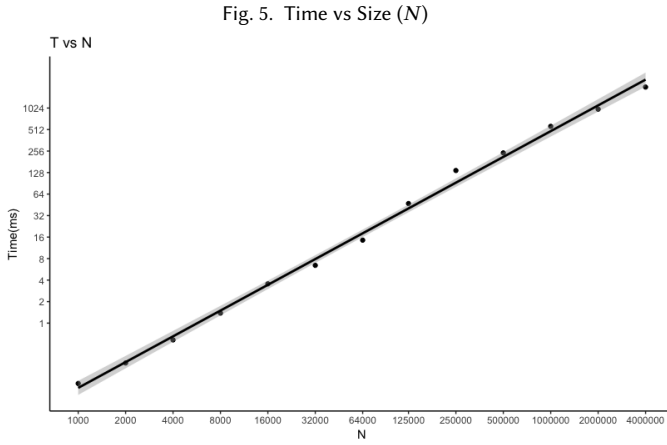
Fig. 5. Time vs Size (N)
