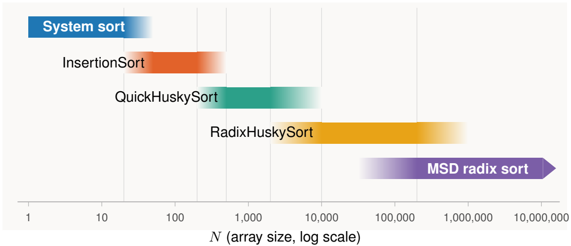
Fig. 5. Which sort to reach for on English text, by array size. Band edges fade across the interval each crossover is bracketed within. MSD radix sort appears because from N = 200,000 it outperforms every husky variant (§ 3.2); it was not in the small- N run, so its band begins at N = 32,000 , where it is level with RadixHuskySort. If instead the data defeats the encoding’s capture window, System sort is the right choice at any N (§ A.2). Band edges fade across the measured crossover zones rather than showing a hard cutoff, reflecting the genuine uncertainty in exactly where each crossover falls. Not shown: if the source data defeats the husky encoding’s fixed capture window, plain System sort is the safe choice at any N (§ A.2); and given a large workload and spare cores, ParallelRadixHuskySort extends RadixHuskySort’s own advantage further still (§ 6.4).
