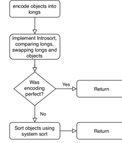
Figure 3.1: HuskySort Flow
