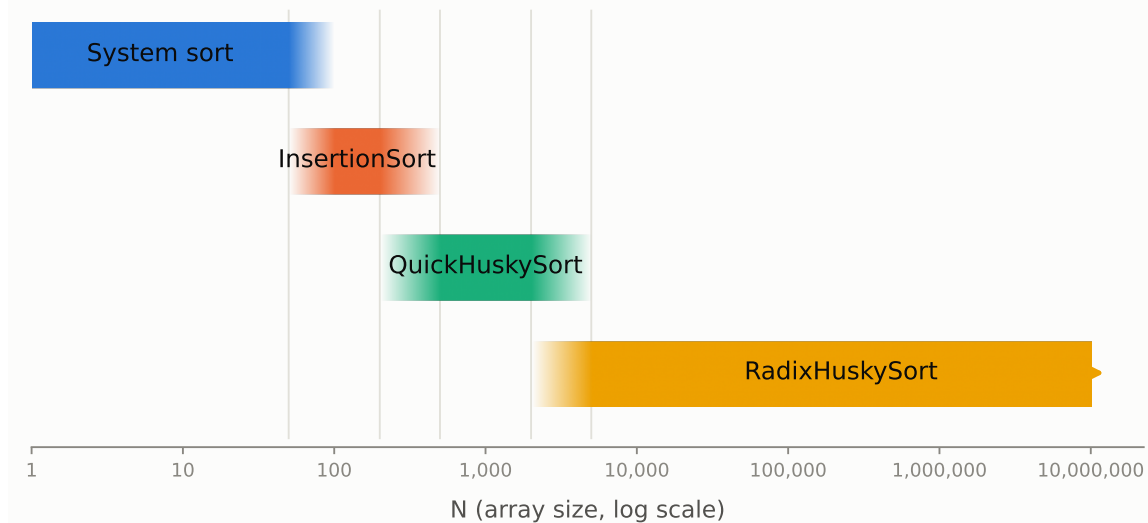
Fig. 5. Which sort to reach for, by array size (String keys). Band edges fade across the measured crossover zones rather than showing a hard cutoff, reflecting the genuine uncertainty in exactly where each crossover falls. Not shown: if the source data defeats the husky encoding’s fixed capture window, plain System sort is the safe choice at any N (§ A.2); and given a large workload and spare cores, ParallelRadixHuskySort extends RadixHuskySort’s own advantage further still (§ 6.4).
