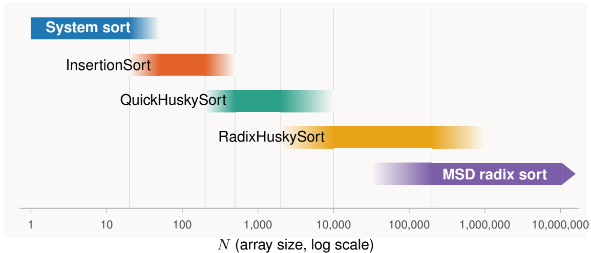
Fig. 5. Which sort to reach for on English text, by array size. Band edges fade across the interval within which each crossover is bracketed, rather than showing a hard cutoff. MSD radix sort appears because from N = 200,000 it outperforms every husky variant (§ 3.2); it was not in the small- N run, so its band begins at N = 32,000 , where it is level with RadixHuskySort. Not shown: if the data defeats the encoding’s capture window, System sort is the right choice at any N (§ A.2); and given a large workload and spare cores, ParallelRadixHuskySort extends RadixHuskySort’s advantage further still (§ 6.4).
