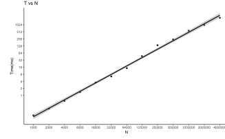
Fig. 4. Time vs Size ( N )
