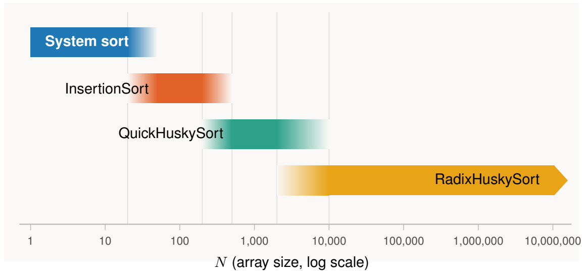
Fig. 5. Which sort to reach for, by array size (String keys). Band edges fade across the measured crossover zones rather than showing a hard cutoff, reflecting the genuine uncertainty in exactly where each crossover falls. Not shown: if the source data defeats the husky encoding’s fixed capture window, plain System sort is the safe choice at any N (§ A.2); and given a large workload and spare cores, ParallelRadixHuskySort extends RadixHuskySort’s own advantage further still (§ 6.4).
