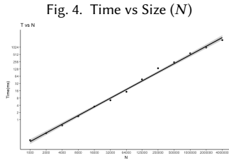
Fig. 4. Time vs Size ( N )
