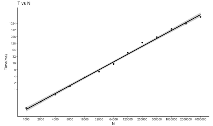
Fig. 4. Time vs Size ( N )
