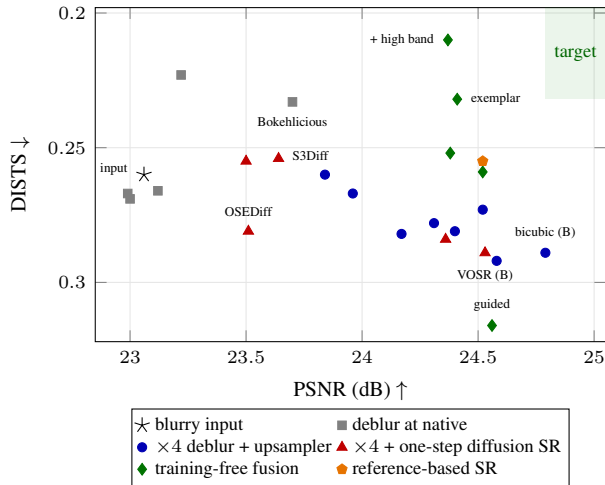
Figure 3. Fidelity vs. perceptual quality of existing approaches at native resolution (76 scenes; up and right is better). Every baseline lies on or below one trade-off curve between the most faithful pipeline ( \times 4 Bokehlicious + bicubic, perceptually worse than the input) and fusions that add the input’s high band. The shaded region, the fidelity of the best low-resolution pipeline with the texture of the non-learned exemplar transfer, is empty. (B): Bokehlicious anchor, otherwise DRBNet. METHOD points.
