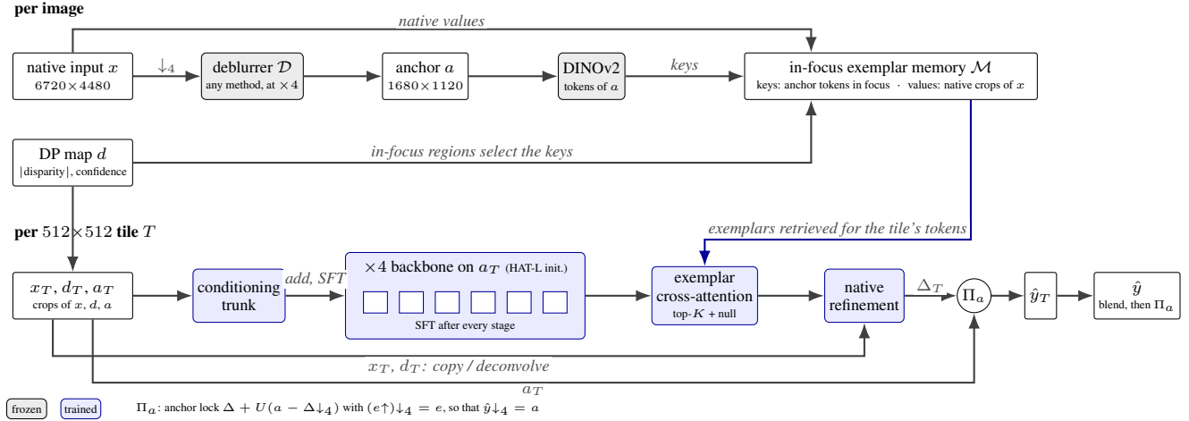
Figure 2. Overview. Per image : any deblurring method \mathcal{D} produces the anchor a at 4\times lower resolution; DINOv2 features of the anchor index the in-focus regions (from the dual-pixel map d ) into a memory whose values are native crops of the observation x . Per tile : the native crop x_T and d_T condition every stage of a \times 4 network applied to the anchor tile; exemplars retrieved for the tile’s tokens enter through cross-attention (with a null option); a native refinement sees x_T directly. The anchor lock \Pi_a keeps the result’s \times 4 band equal to the anchor, per tile and again after blending.
