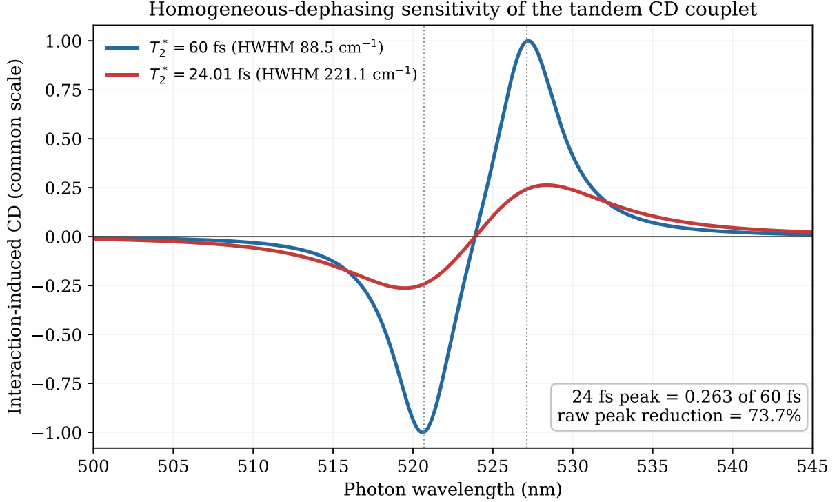
Figure 2: Project-generated 60 fs and 24.01 fs tandem CD differences on a shared amplitude scale. Dotted lines mark the mean exciton centres. The faster-dephasing curve is broader and has only 26.3% of the raw 60 fs peak.
