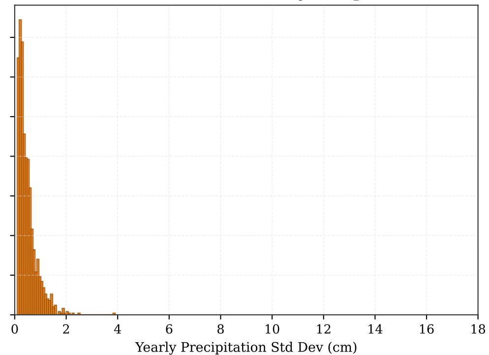
Standard Deviation of Yearly Precipitation
