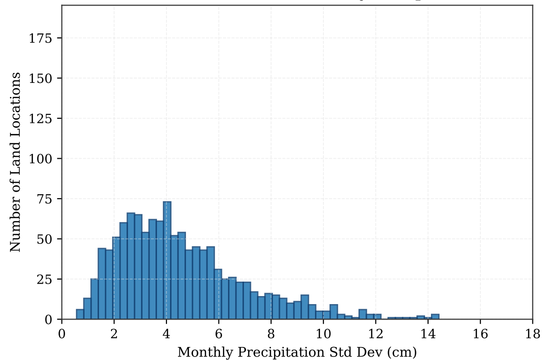
Standard Deviation of Monthly Precipitation
