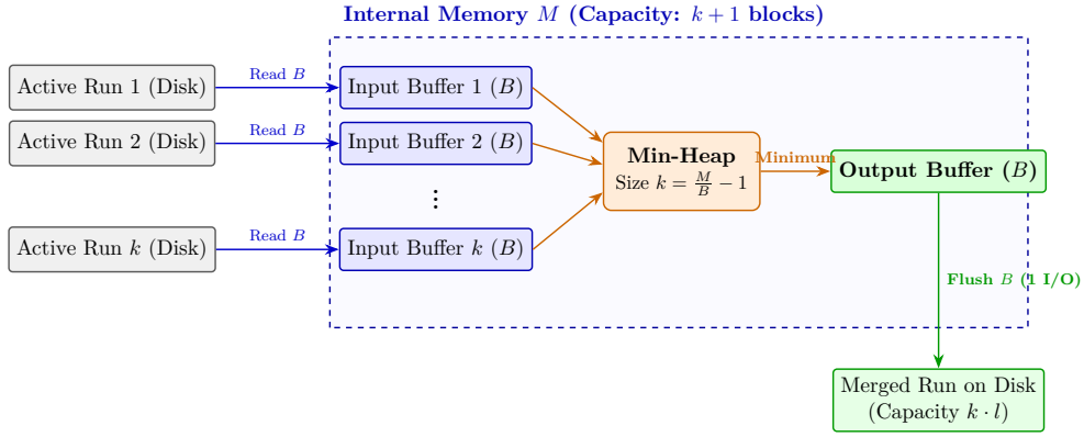
Figure 4.1: Internal memory layout during multiway merging ( k -Way Merge Sort) with coordinating Min-Heap.
