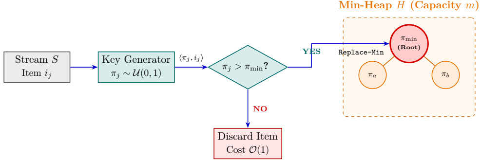
Figure 8.2: Functional flow of streaming Priority Sampling using a bounded Min-Heap of capacity m .
