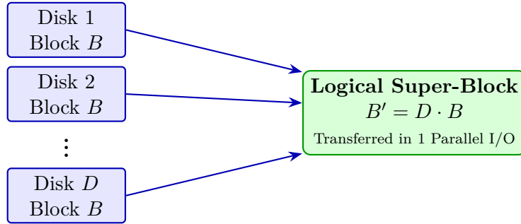
Figure 4.4: Disk striping layout: aggregating D physical blocks into a single logical super-block B' .
