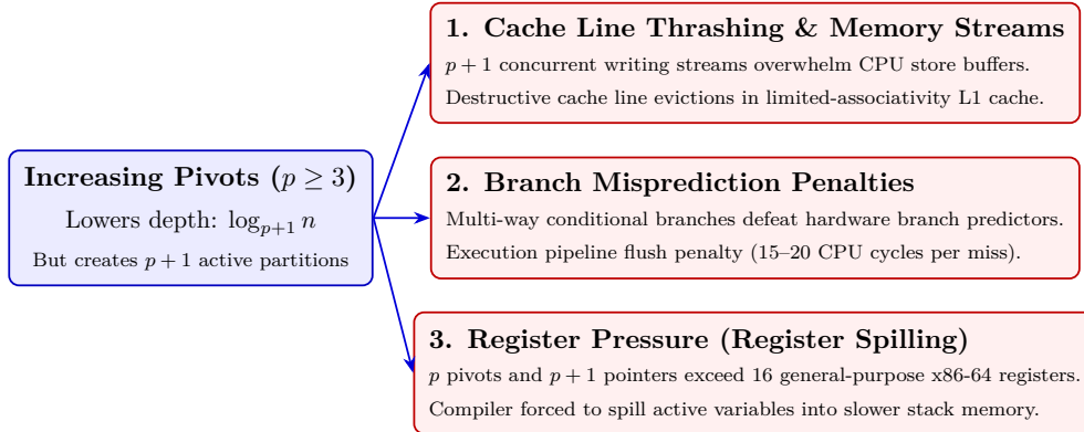
Figure 6.2: Microarchitectural degradation mechanisms caused by increasing the pivot count p .
