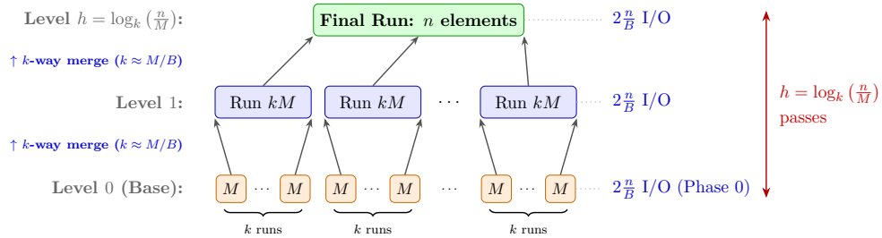
Figure 4.2: Level evolution and k -way merge tree in Multiway Merge Sort.
