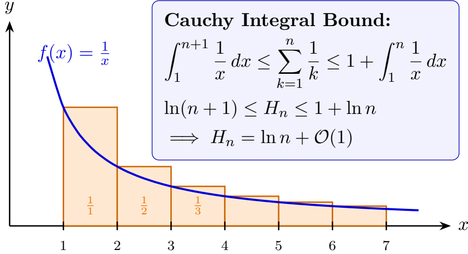
Figure 6.4: Integral approximation of the harmonic series H_n = \sum_{k=1}^n \frac{1}{k} \approx \ln n . The rectangle areas upper-bound the integral of the hyperbola f(x) = \frac{1}{x} .
