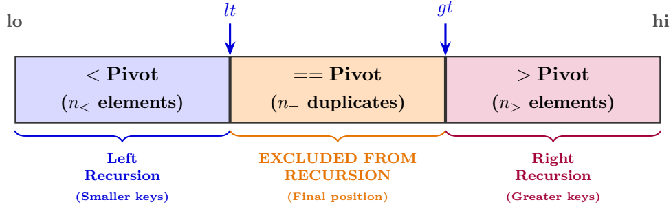
Figure 6.3: Topology of the three regions in 3-way partitioning ( Dutch National Flag ) and boundary pointers lt and gt .
