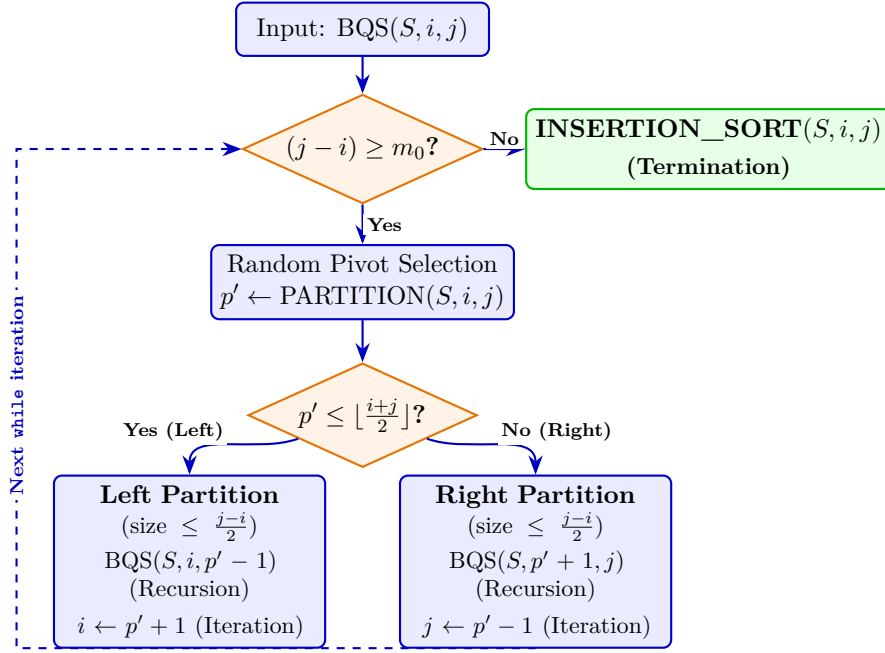
Figure 5.4: Control flow of Bounded Quicksort (BQS). Recursive invocations are strictly bounded to the smaller partition ( \leq (j - i)/2 ), while the larger half is evaluated iteratively inside the while loop. Partitions smaller than m_0 are sorted directly via Insertion Sort.
