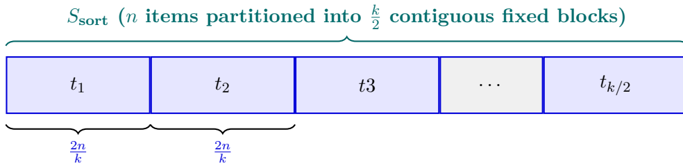
Figure 7.3: Theoretical partitioning of S_{\text{sort}} into \frac{k}{2} fixed blocks t_j of size \frac{2n}{k} .
