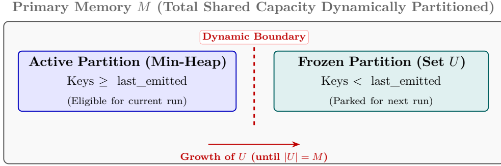
Figure 4.3: Dynamic partitioning of memory M during Replacement Selection (Snow Plow).
