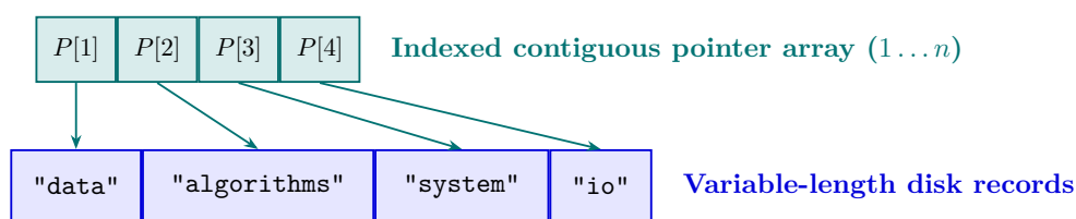
Figure 7.4: Mapping variable-length string records using a contiguous indexed pointer array.
