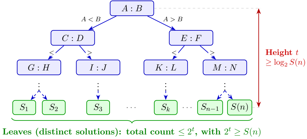
Figure 5.1: Binary decision tree model for comparison-based algorithms. Internal nodes represent elementary pairwise comparisons; leaves represent admissible distinct solutions (S_1, S_2, \dots, S(n)) . The longest path determines the worst-case running time.
