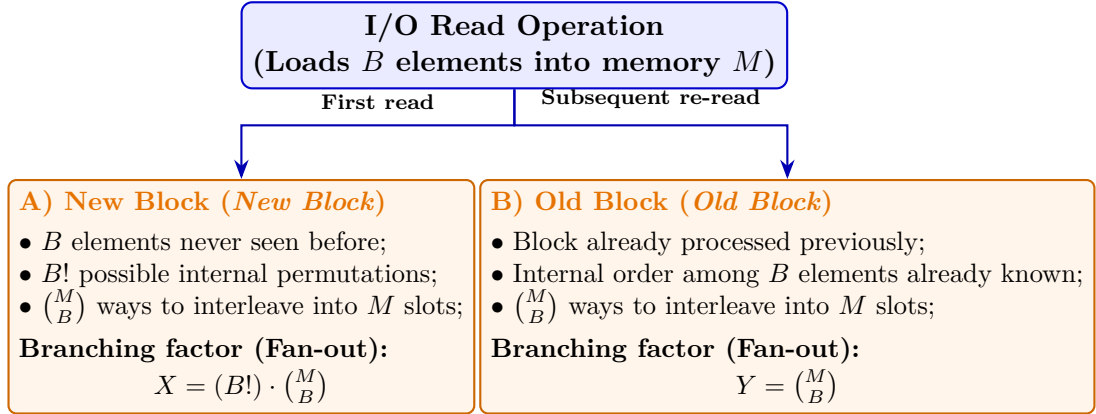
Figure 5.2: Branching factors ( fan-out ) in the I/O decision tree under the two-level memory model: reading a new block yields internal order information ( B! ) and interleaving information ( \binom{M}{B} ); re-reading an old block yields only interleaving information.
