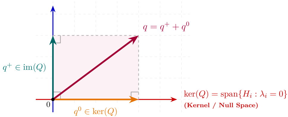
Figure 9.1: Orthogonal subspace decomposition \mathbb{R}^n = \text{im}(Q) \oplus \text{ker}(Q) : the linear term vector q decomposes uniquely into the sum q = q^+ + q^0 , with q^+ \perp q^0 .
