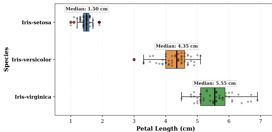
Figure 2.2: Conditional Box Plot computed on the real Iris dataset: empirical distribution of Petal Length stratified across the three flower species, displaying median, quartiles, and individual observations.
