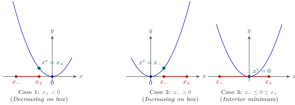
Figure 7.1: The three topological configurations for box-constrained homogeneous quadratic optimization over [x_-, x_+] .
