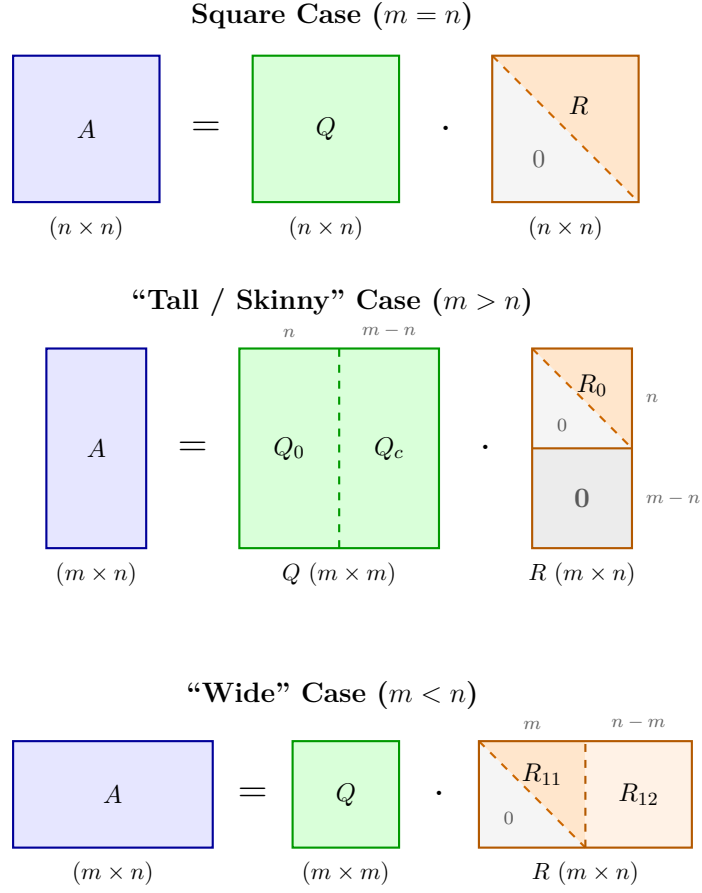
Figure 6.1: Dimensional structure of the QR decomposition across the three geometric regimes ( m = n , m > n , and m < n ).
