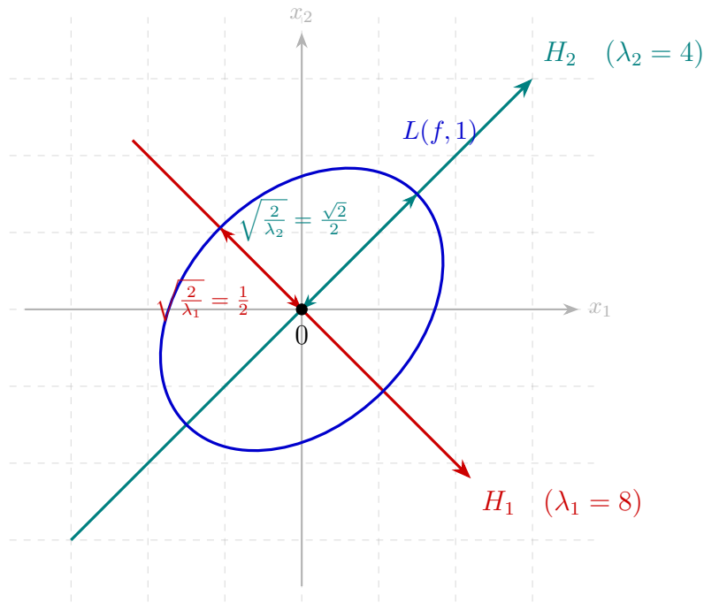
Figure 8.3: Geometry of level set L(f, 1) for a positive definite matrix: alignment along orthonormal eigenvectors H_1, H_2 and inverse semi-axis proportionality.
