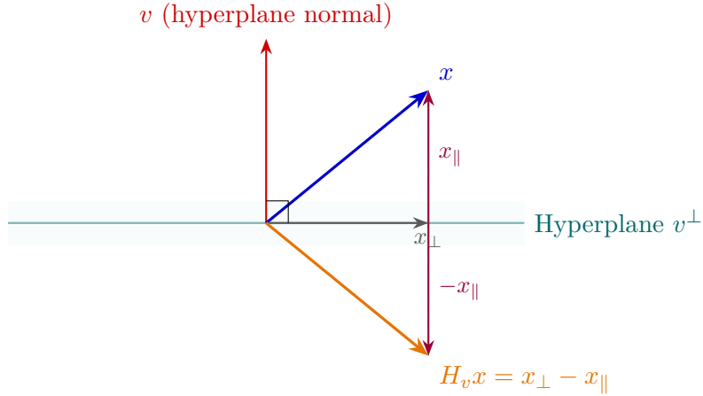
Figure 6.2: Geometric interpretation of a Householder reflection: specular reflection across the hyperplane v^\perp .
