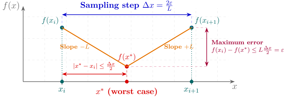
Figure 11.2: Worst-case error analysis for uniform sampling: if f is L -Lipschitz, in the worst case the minimum x^* lies at the midpoint \Delta x/2 , bounding function value error by L\frac{\Delta x}{2} \leq \varepsilon .
