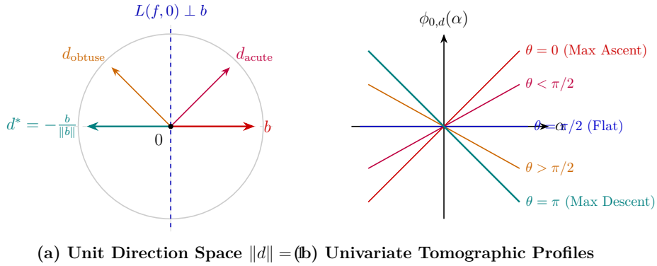
Figure 8.2: Tomographic inspection of a linear function: rotating search directions and identifying slope bounds.
