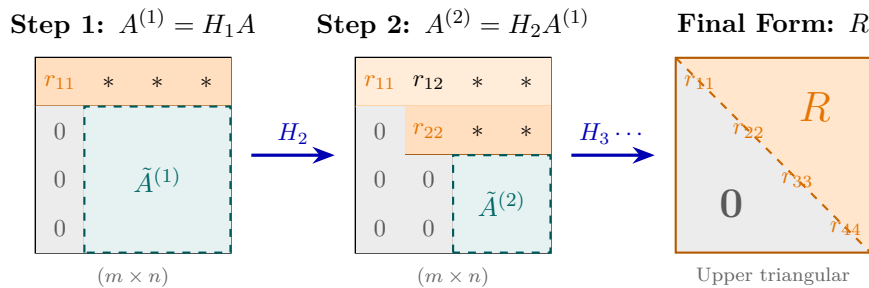
Figure 6.3: Iterative subdiagonal zeroing via the Householder QR algorithm.
