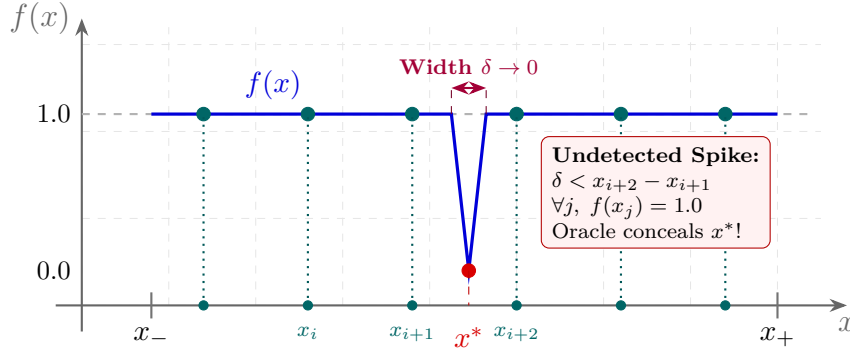
Figure 11.1: The pathology of narrow continuous spikes: even on a compact interval [x_-, x_+] , a continuous function can plummet to its minimum across a base \delta narrower than the distance between adjacent samples, evading any finite grid.
