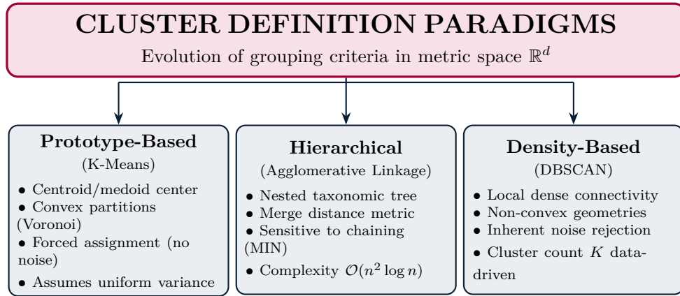
Figure 8.1: Conceptual positioning of density-based clustering relative to prototype-based and hierarchical paradigms.
