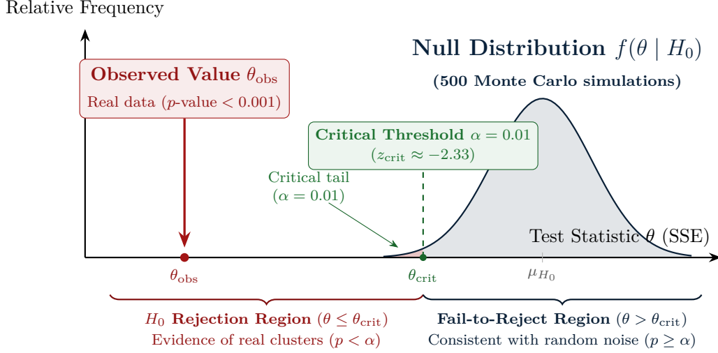
Figure 10.5: Null model hypothesis testing framework: when observed SSE falls far to the left of the empirical null distribution, the randomness hypothesis is formally rejected.
