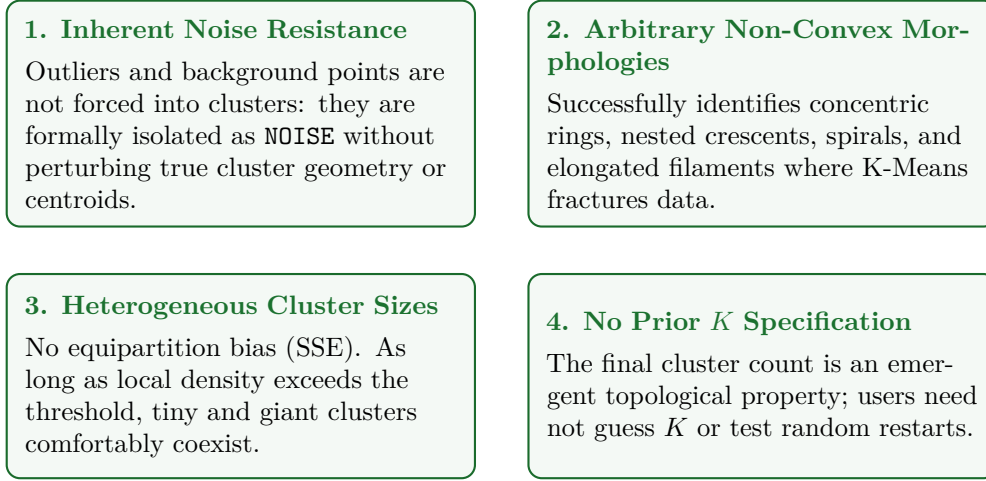
Figure 8.5: Four key architectural strengths of DBSCAN over prototype-based models.
