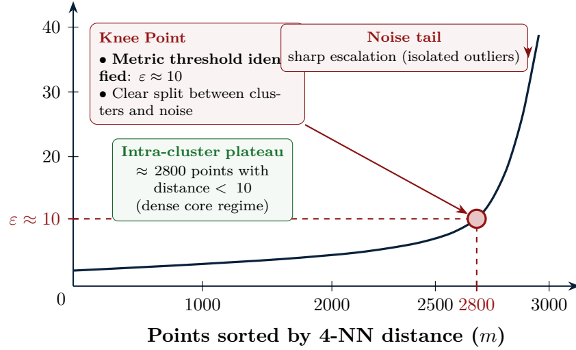
Figure 8.7: The k -distance plot ( k = 4 ) for approximately 3000 points. The optimal radius threshold \epsilon is identified at the knee point along the Y-axis, here located at \epsilon \approx 10 .
