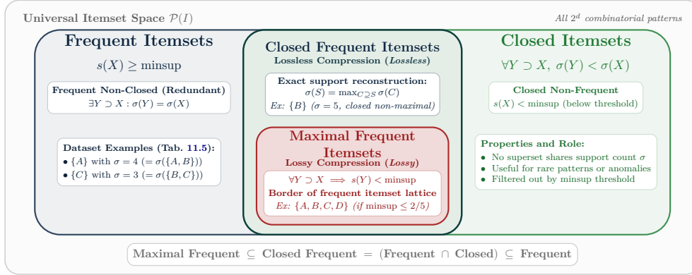
Figure 11.4: Euler-Venn diagram illustrating inclusion relationships between frequent, closed, and maximal itemsets, highlighting lossless vs lossy compression characteristics.
