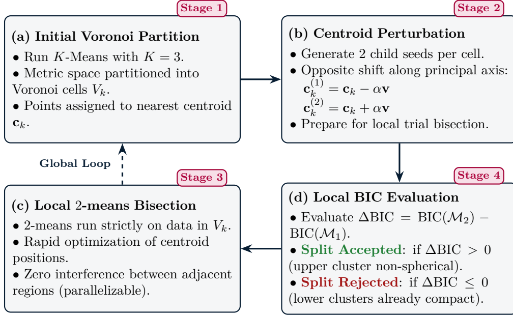
Figure 9.3: Four-stage operational cycle of X-Means: initial Voronoi partition, directional seed perturbation, local bisection, and statistical validation via the information-theoretic \Delta\text{BIC} test.
