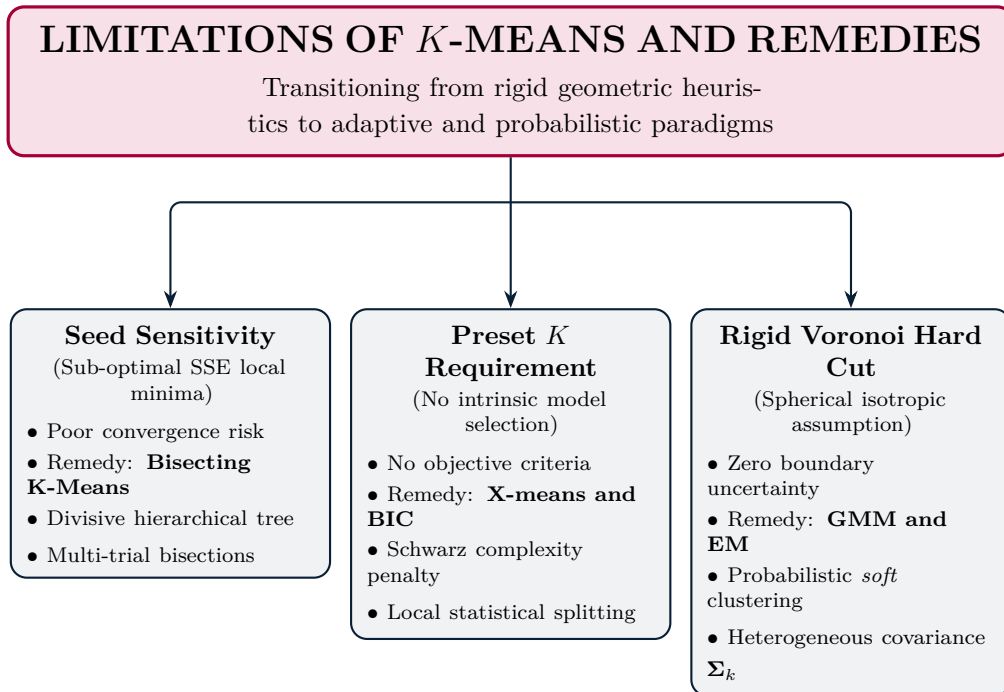
Figure 9.1: Conceptual overview of the foundational limitations of standard K -Means and the three complementary algorithmic strategies designed to address them.
