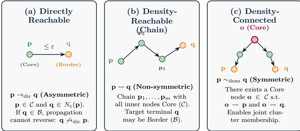
Figure 8.3: Algebraic formalization of the three density spatial relations in DBSCAN.
