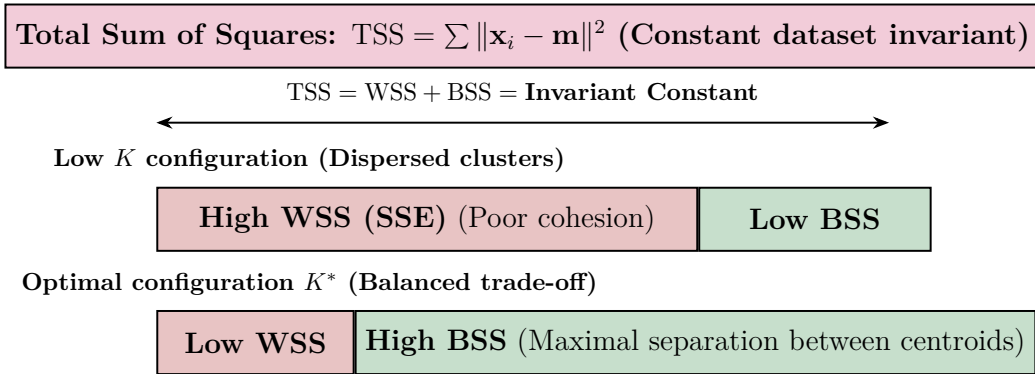
Figure 10.3: Total variance conservation decomposition \text{TSS} = \text{WSS} + \text{BSS} : minimizing within-cluster dispersion WSS is mathematically identical to maximizing between-cluster separation BSS.
