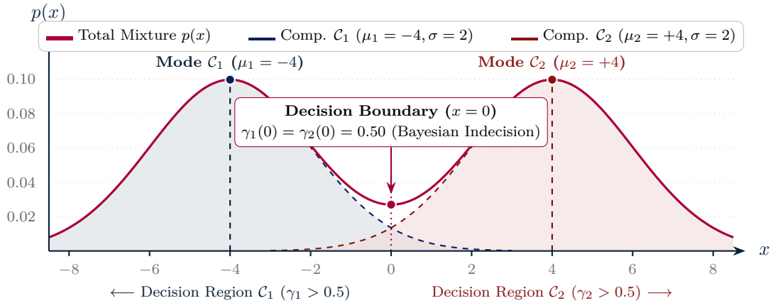
Figure 9.5: Analytical deconvolution of a bimodal two-Gaussian mixture with equal variance ( \sigma = 2 ) and separated centers ( \Delta\mu = 8 ).
