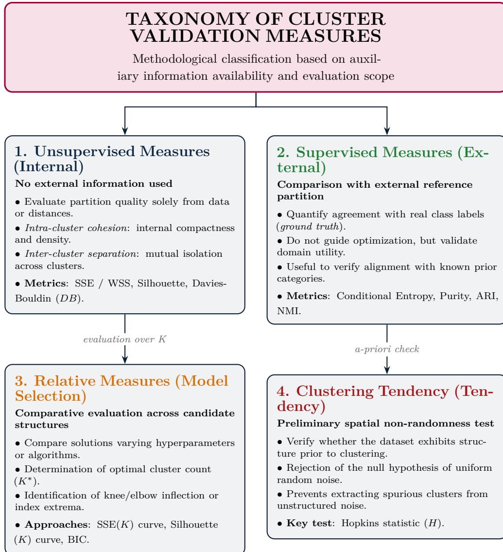
Figure 10.1: Taxonomy of cluster validation measures categorized by data nature and analytical objective.
