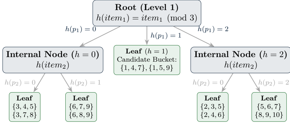
Figure 11.2: Hash tree indexing architecture for efficient candidate support counting.
