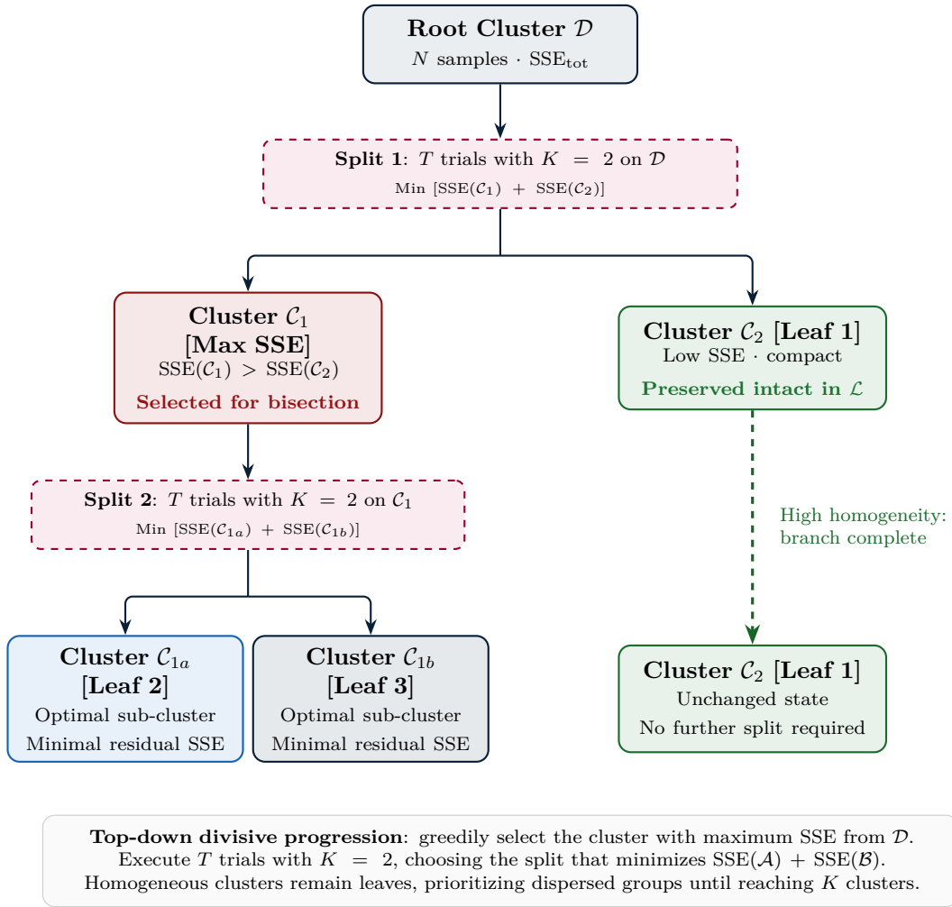
Figure 9.2: Hierarchical binary tree representation of the divisive progression of Bisecting K -Means with multiple bisection trials and minimum SSE selection.
