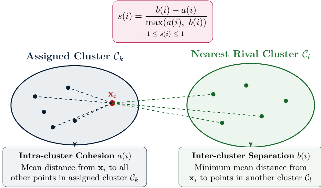
Figure 10.4: Silhouette coefficient geometry: visual comparison between internal cohesion a(i) and separation from the nearest rival cluster b(i) .
