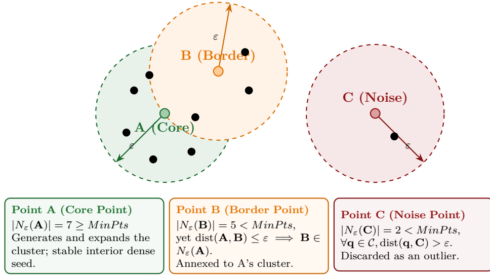
Figure 8.2: Geometric taxonomy of points in DBSCAN ( \text{MinPts} = 7 ). Point A is a Core Point ( |N_\varepsilon(A)| \geq 7 ), B is a Border Point ( |N_\varepsilon(B)| < 7 , but within radius \varepsilon of core A), and C is Noise (isolated, far from all cores).
