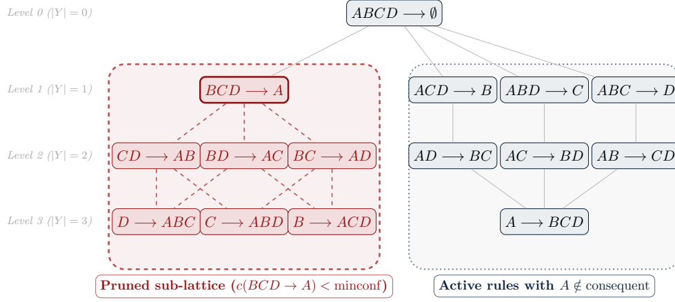
Figure 11.3: Rule lattice generated from \{A, B, C, D\} organized by consequent cardinality ( |Y| ). As soon as rule BCD \rightarrow A falls below \text{minconf} , all of its descendants (having A in their consequent, highlighted on the left) are pruned a priori by confidence anti-monotonicity.
