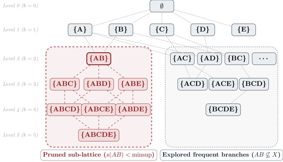
Figure 11.1: Itemset lattice representation for d = 5 items. As soon as \{AB\} is found infrequent ( s(AB) < \text{minsup} ), the entire sub-lattice of its 2^{5-2} = 8 supersets (highlighted on the left in red) is pruned a priori , while the remaining branches not containing \{AB\} (on the right) continue to be explored.
