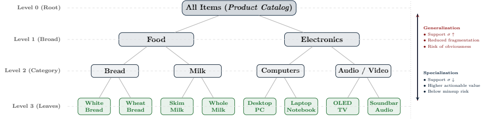
Figure 11.5: Multi-level conceptual taxonomy for hierarchical association rule mining, highlighting taxonomy levels and the generalization vs. specialization trade-off.
