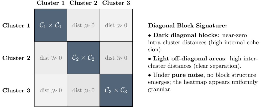
Figure 10.2: Reordered distance matrix schematic: prominent square blocks along the main diagonal visually confirm cluster validity.
