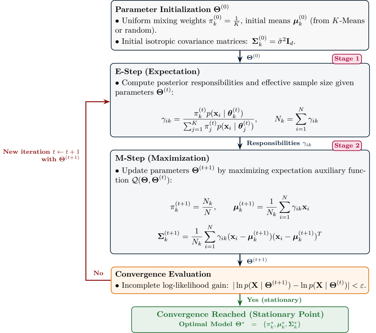
Figure 9.4: Operational flowchart of the Expectation-Maximization (EM) algorithm.
