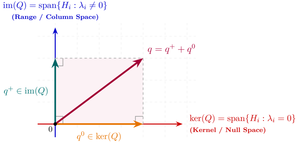
Figure 9.1: Orthogonal subspace decomposition \mathbb{R}^n = \text{im}(Q) \oplus \ker(Q) : the linear term vector q decomposes uniquely into the sum q = q^+ + q^0 , with q^+ \perp q^0 .
