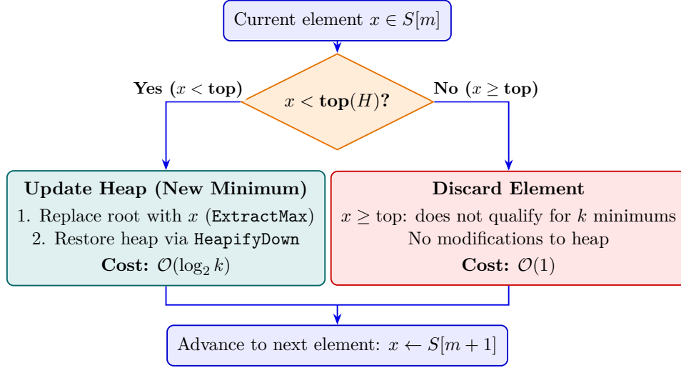
Figure 5.1: Decision flow using a bounded Max-Heap of size k . Elements that do not improve the current k minimums are discarded in constant time \mathcal{O}(1) .
