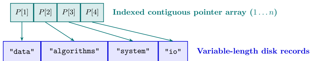
Figure 6.4: Mapping variable-length string records using a contiguous indexed pointer array.
