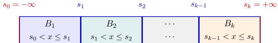
Figure 6.1: Partitioning of dataset S into k buckets using k - 1 sorted pivots.
