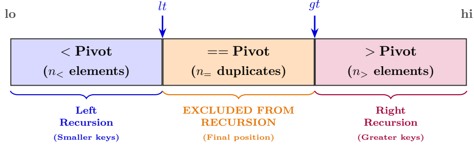
Figure 5.3: Topology of the three regions in 3-way partitioning ( Dutch National Flag ) and boundary pointers lt and gt .
