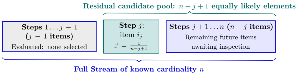
Figure 7.1: Stream space partition at step j for single-element sampling ( m = 1 ).
