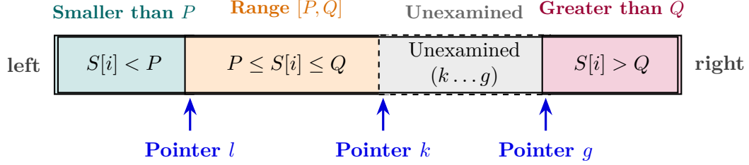
Figure 4.3: Dual-Pivot Quicksort partitioning schema (Yaroslavskiy). The array is partitioned into four dynamic regions: elements < P , elements between P and Q , unexamined elements between k and g , and elements > Q .
