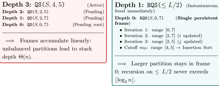
Figure 4.5: Execution trace of Bounded Quicksort (BQS) with threshold m_0 = 3 and call stack memory comparison. (A) At each iteration, the larger partition is processed within the same stack frame by updating i or j , while only the halved partition ( \leq L/2 ) triggers a short-lived recursive call. (B) Standard Quicksort accumulates call frames linearly; BQS strictly guarantees logarithmic stack depth.
