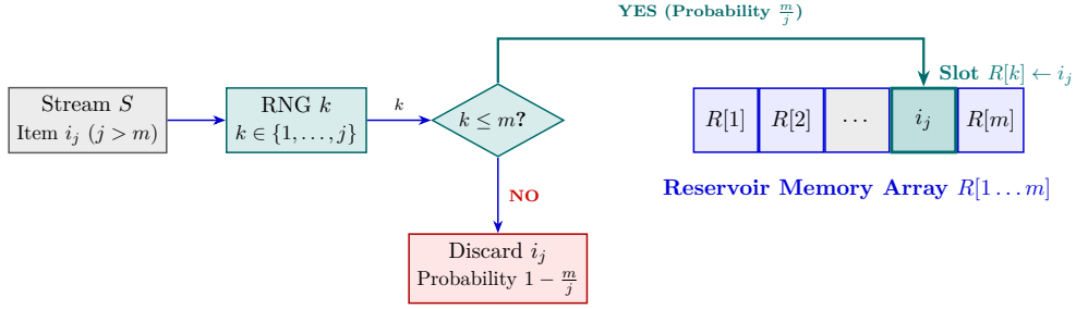
Figure 7.3: Operational replacement flow of Reservoir Sampling (Algorithm R).
