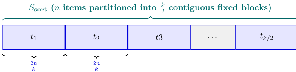
Figure 6.3: Theoretical partitioning of S_{\text{sort}} into \frac{k}{2} fixed blocks t_j of size \frac{2n}{k} .
