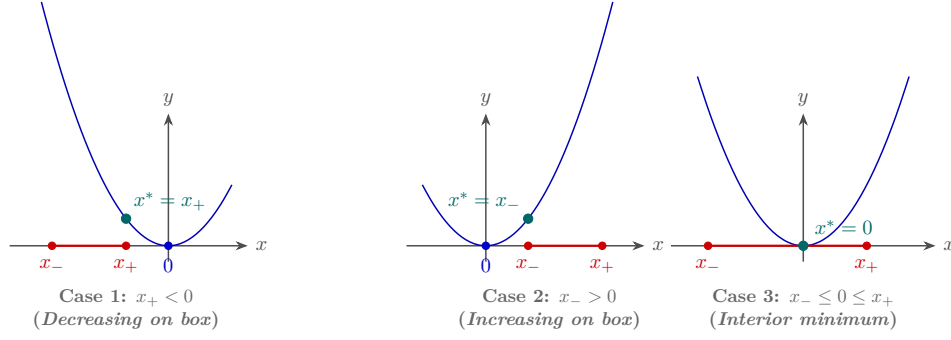
Figure 5.1: The three topological configurations for box-constrained homogeneous quadratic optimization over [x_-, x_+] .
