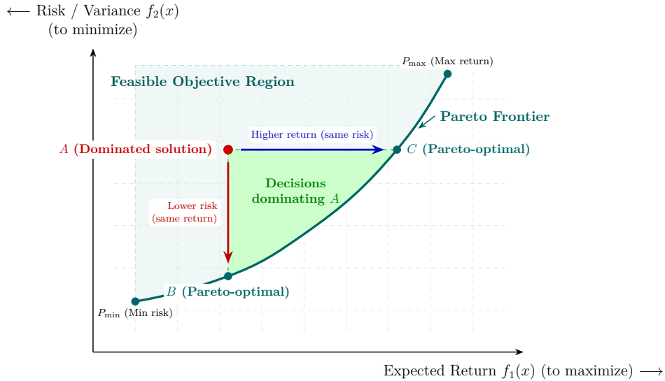
Figure 6.1: Geometric representation of the Pareto Frontier in Markowitz portfolio selection.
