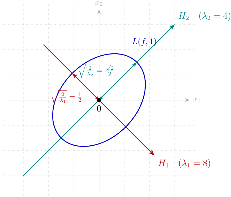
Figure 6.3: Geometry of level set L(f,1) for a positive definite matrix: alignment along orthonormal eigenvectors H_1, H_2 and inverse semi-axis proportionality.
