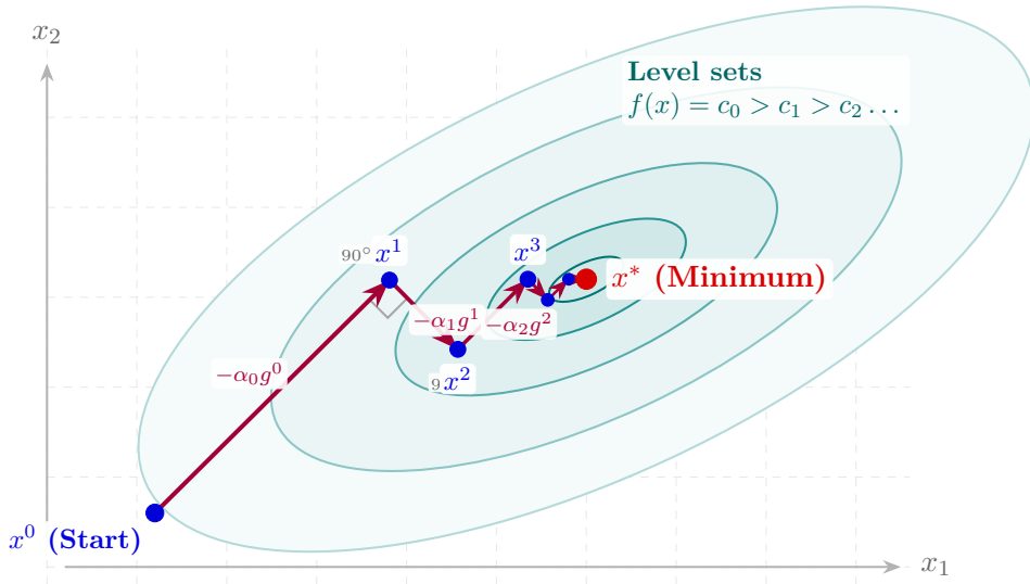
Figure 7.2: Zig-zag trajectory of GMQ across elliptical level sets: exact line search enforces strict orthogonality between successive directions ( \langle g^{k+1}, g^k \rangle = 0 ), constraining iterates to turn at exact right angles ( 90^\circ ).
