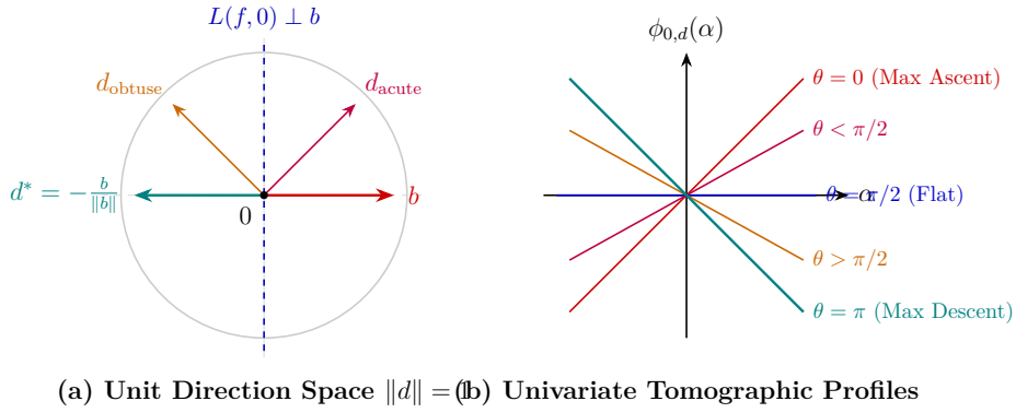
Figure 6.2: Tomographic inspection of a linear function: rotating search directions and identifying slope bounds.
