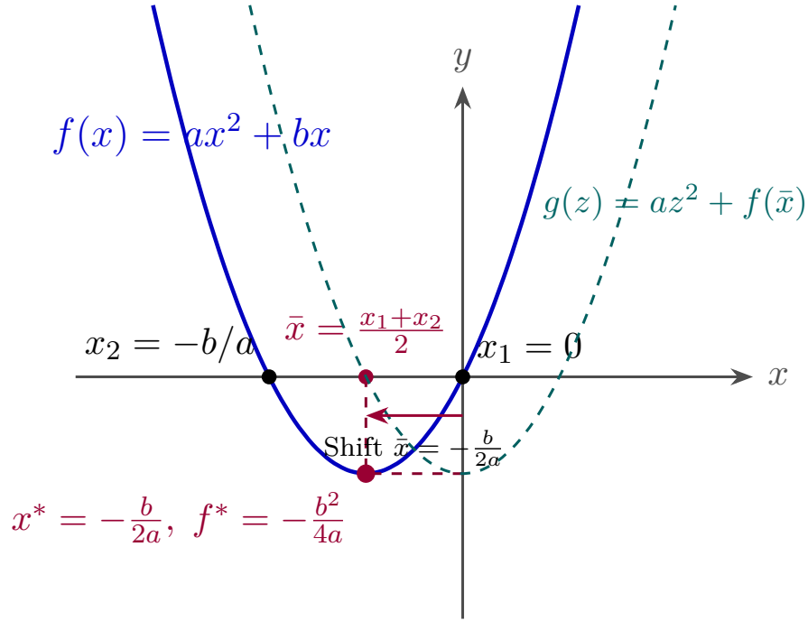
Figure 5.2: Geometric visualization of coordinate translation for the non-homogeneous parabola: the vertex x^* lies precisely at the midpoint between the two roots x_1 and x_2 .
