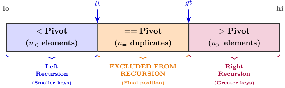
Figure 5.3: Topology of the three regions in 3-way partitioning ( Dutch National Flag ) and boundary pointers lt and gt .
