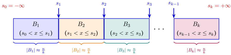
Figure 6.1: Key universe partitioning into k disjoint buckets using k - 1 sorted pivots and two conceptual sentinel boundaries.
