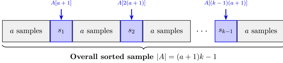
Figure 6.2: Layout of sorted auxiliary array A : exactly a intermediate sample items lie between any two consecutive pivots.
