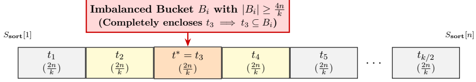
Figure 6.3: Geometric containment construction: any bucket B_i with size \geq 4n/k spans across and fully encloses at least one segment t^* \subset S_{\text{sort}} of width 2n/k .
