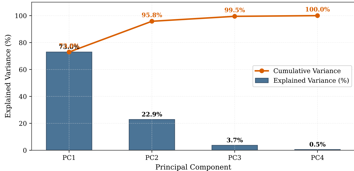
Explained Variance by Principal Component (Scree Plot)
