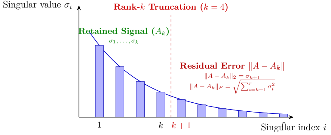
Figure 5.2: Singular spectrum decay and energy partitioning between retained signal ( A_k ) and discarded residual error quantified by the Eckart-Young Theorem.
