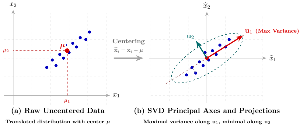
Figure 5.4: Geometric interpretation of PCA via SVD: (a) Original raw data with center \boldsymbol{\mu} ; (b) Centered data with principal directions \mathbf{u}_1 (maximal variance) and orthogonal \mathbf{u}_2 obtained from the SVD of \hat{A} = U \Sigma V^T , displaying orthogonal projections onto the optimal low-rank subspace.
