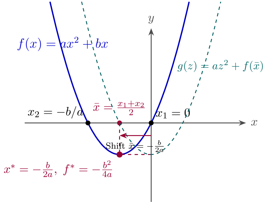
Figure 6.2: Geometric visualization of coordinate translation for the non-homogeneous parabola: the vertex x^* lies precisely at the midpoint between the two roots x_1 and x_2 .
