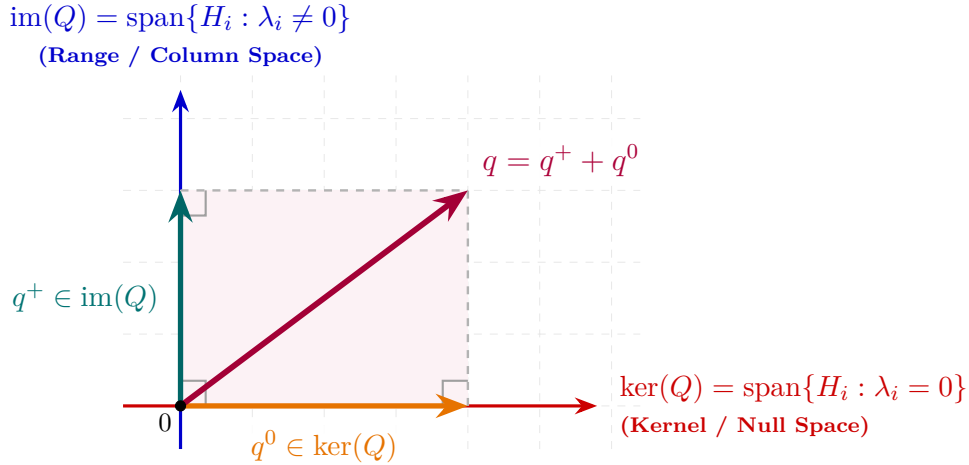
Figure 8.1: Orthogonal subspace decomposition \mathbb{R}^n = \text{im}(Q) \oplus \text{ker}(Q) : the linear term vector q decomposes uniquely into the sum q = q^+ + q^0 , with q^+ \perp q^0 .
