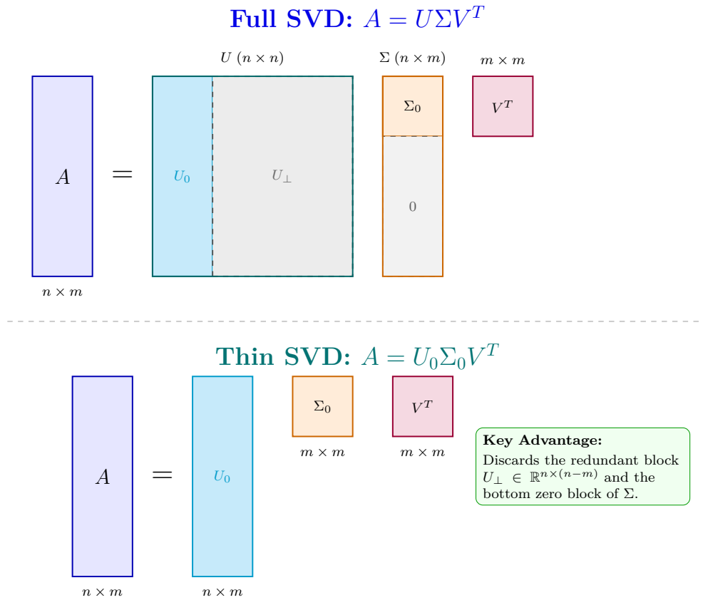
Figure 4.1: Structural and geometric comparison between Full SVD and Thin SVD for a tall and thin matrix ( n > m ).
