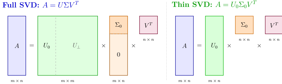
Figure 5.1: Structural and dimensional comparison between Full SVD and Economy (Thin) SVD for tall matrices ( m \geq n ). Thin SVD eliminates the zero rows of \Sigma and the unneeded trailing columns U_\perp .
