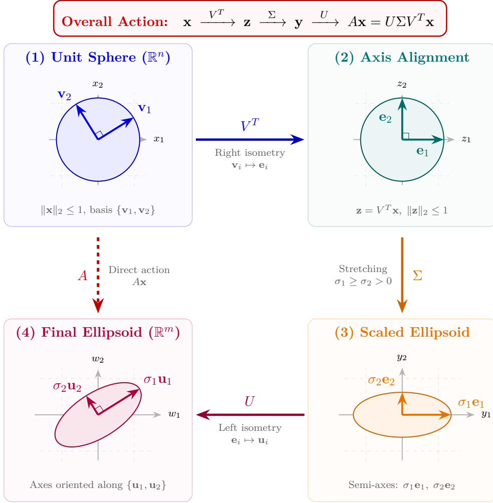
Figure 5.3: Four-quadrant geometric interpretation of the linear mapping A = U\Sigma V^T acting on the unit Euclidean sphere: (1) Initial unit sphere with orthonormal right singular basis \mathbf{v}_i ; (2) Right isometry V^T aligning \mathbf{v}_i to the canonical axes; (3) Axis-aligned dilation \Sigma producing an ellipsoid with semi-axes \sigma_i ; (4) Final left isometry U orienting principal axes along the left singular vectors \mathbf{u}_i .
