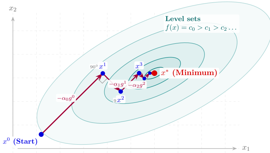
Figure 8.2: Zig-zag trajectory of GMQ across elliptical level sets: exact line search enforces strict orthogonality between successive directions ( \langle g^{k+1}, g^k \rangle = 0 ), constraining iterates to turn at exact right angles ( 90^\circ ).
