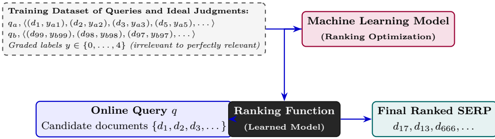
Figure 1.5: Conceptual workflow of Learning-to-Rank (LTR): from training with graded labels to online SERP ordering (Slide 19).
