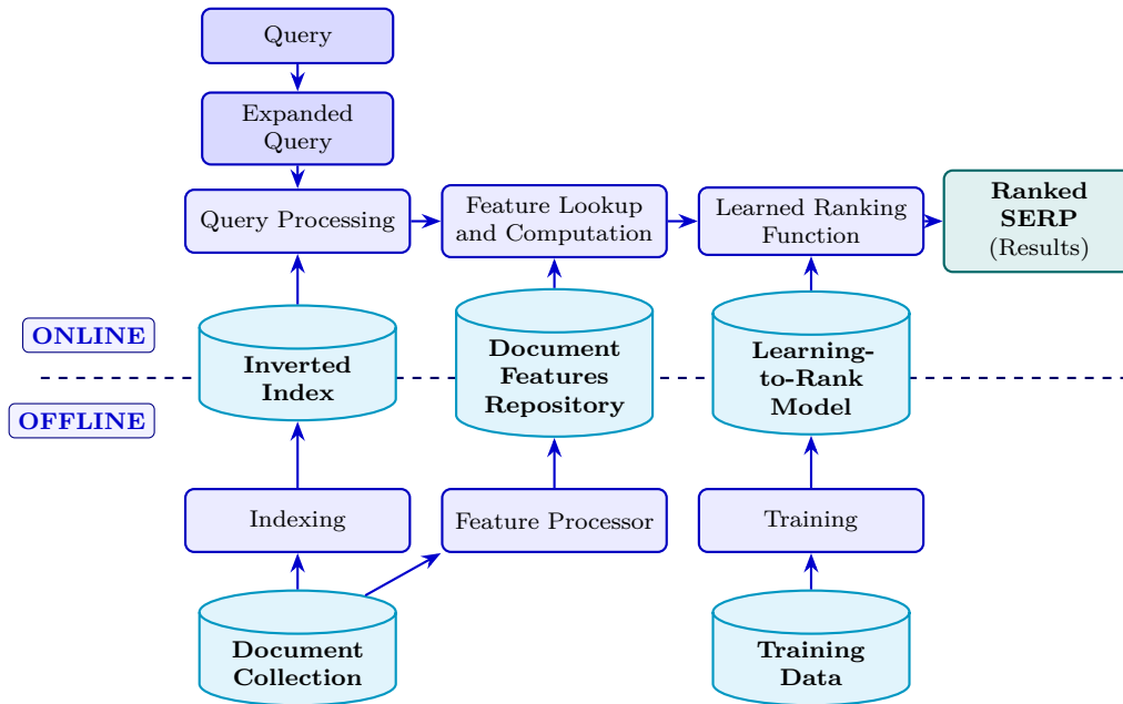
Figure 1.2: Grid architecture of a modern search engine (Online vs. Offline pipelines).
