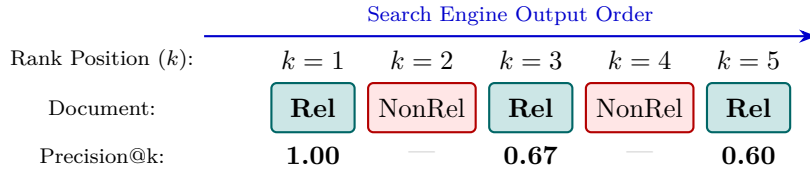
Figure 2.3: Schematic representation of Average Precision calculation over 5 documents with R = 3 total relevant items (Slide 22).
