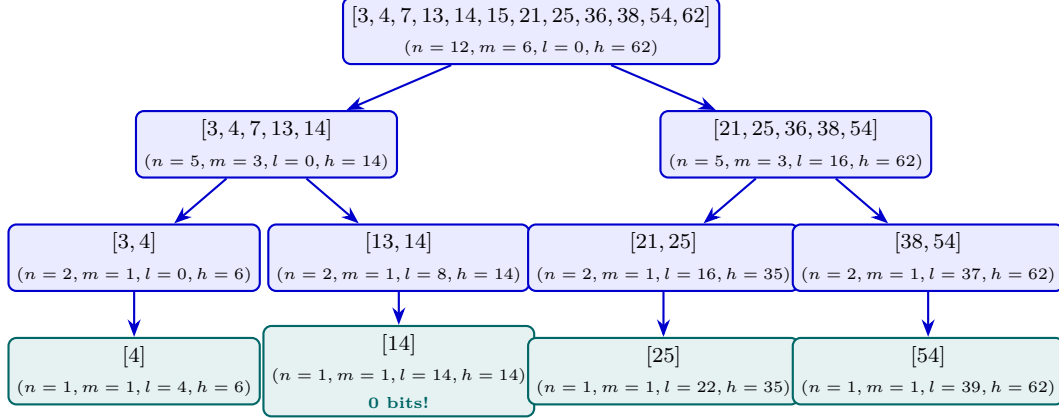
Figure 1.4: Dichotomous decomposition tree for Binary Interpolative Coding (Slide 18).
