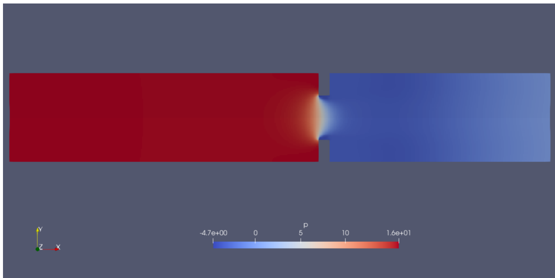
Figure 6: Pressure contours
