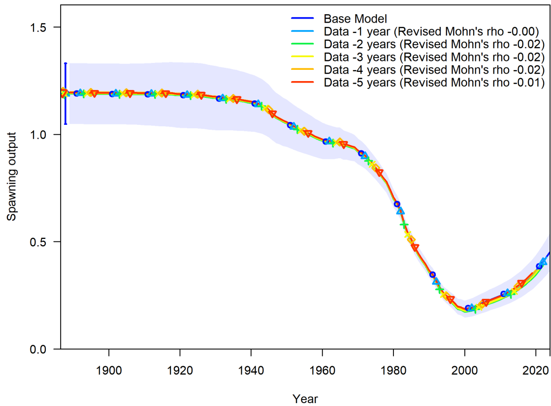
Figure 78: Results of retrospective analysis. Spawning output (billions of eggs) time series of this assesment base model are proved with \sim 95\% interval.
