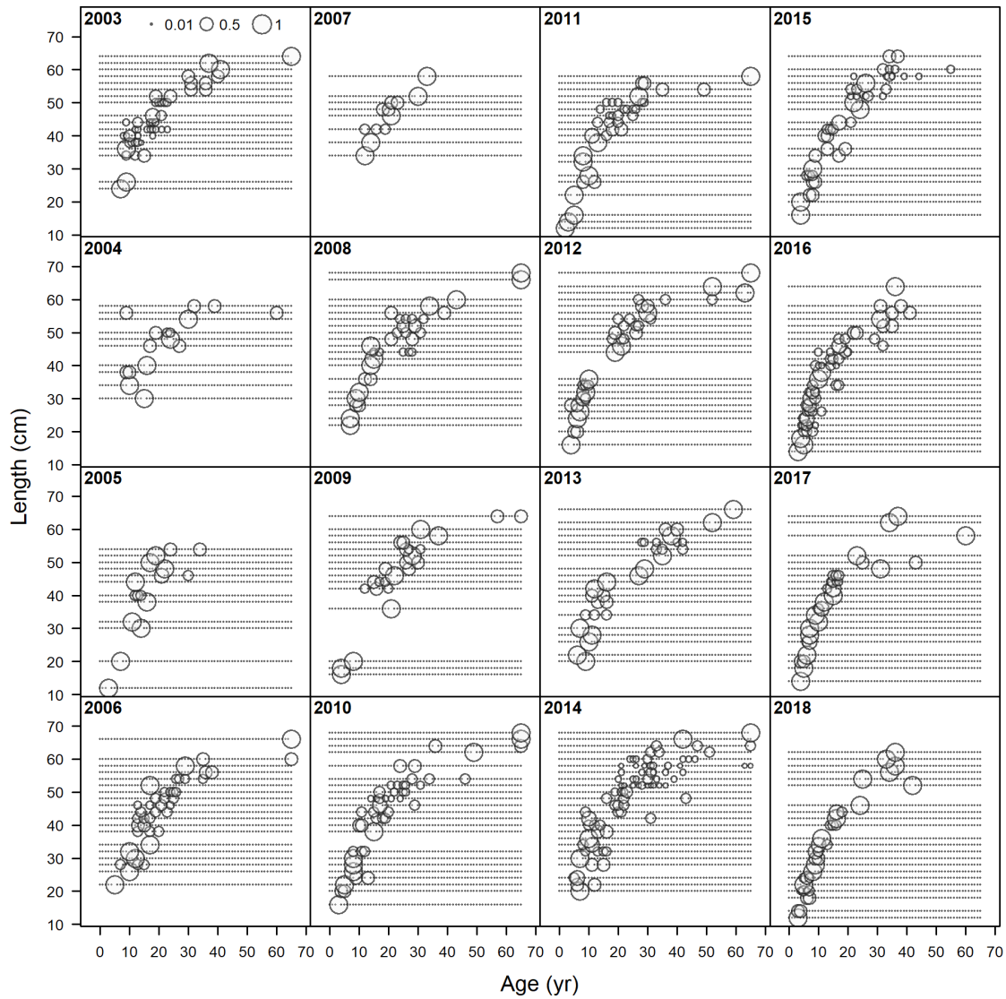
Figure 13: Annual unsexed conditional age-at-length data for the WCGTBTS (1 of 2).
