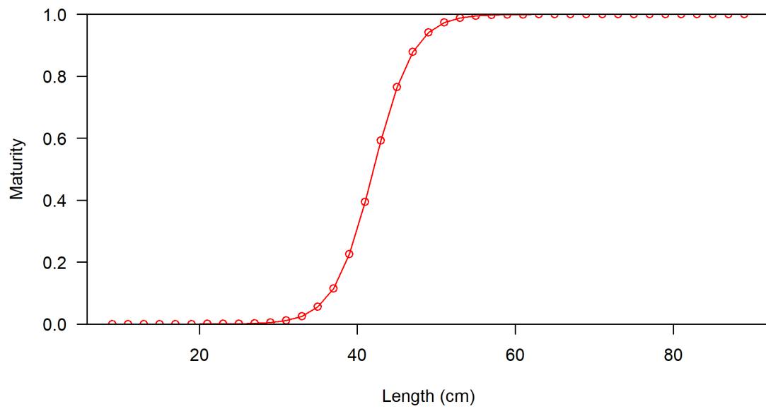
Figure 18: Maturity at length relationship used in the base model for Yelloweye Rockfish.
