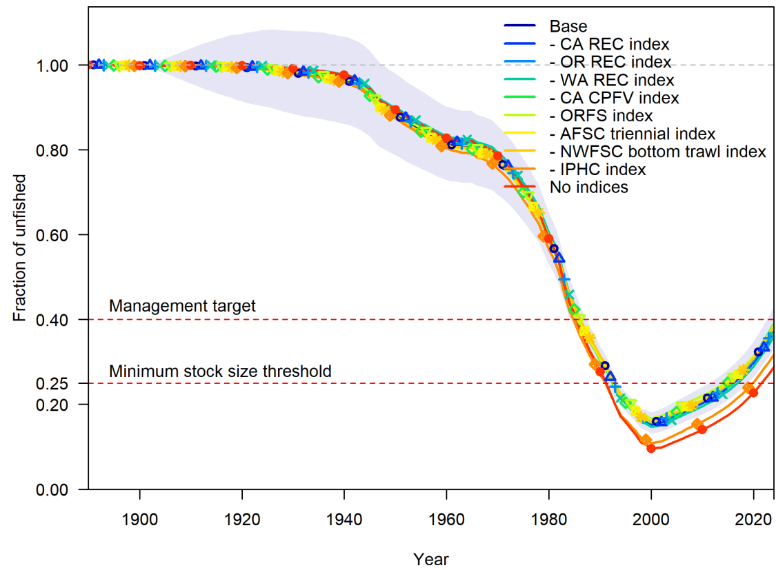
Figure 74: Relative spawning output across index inclusion sensitivities.
