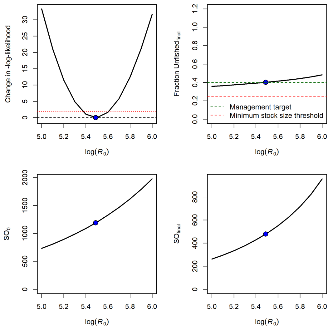
Figure 87: Likelihood profile (top left panel) for log initial recruitment ( \ln R_0 ), with associated changes in stock status in the current year ( SB_{2025}/SB_0 ; top right panel), initial spawning biomass ( SB_0 ; bottom left panel), and current year spawning biomass ( SB_{2025} ; bottom right panel). Points indicate the base model MLE estimate.
