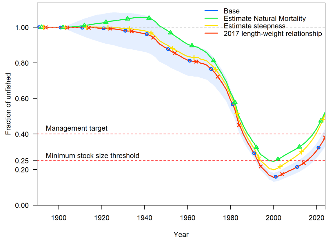
Figure 64: Relative spawning output across model structure sensitivities.
