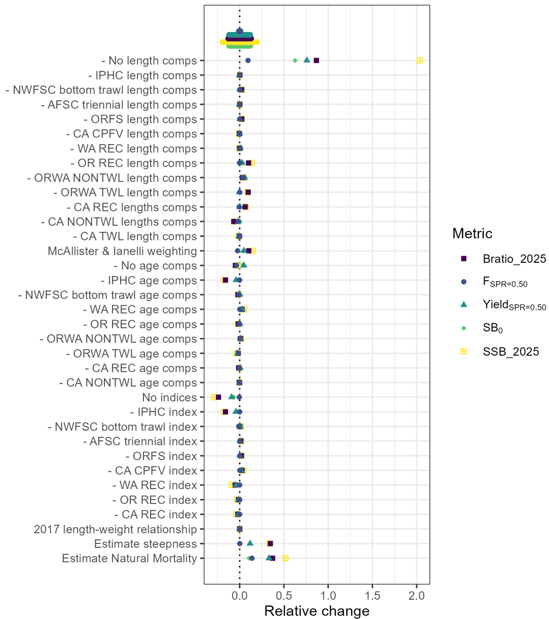
Figure 75: Relative change in management quantities across models conducted as sensitivities.
