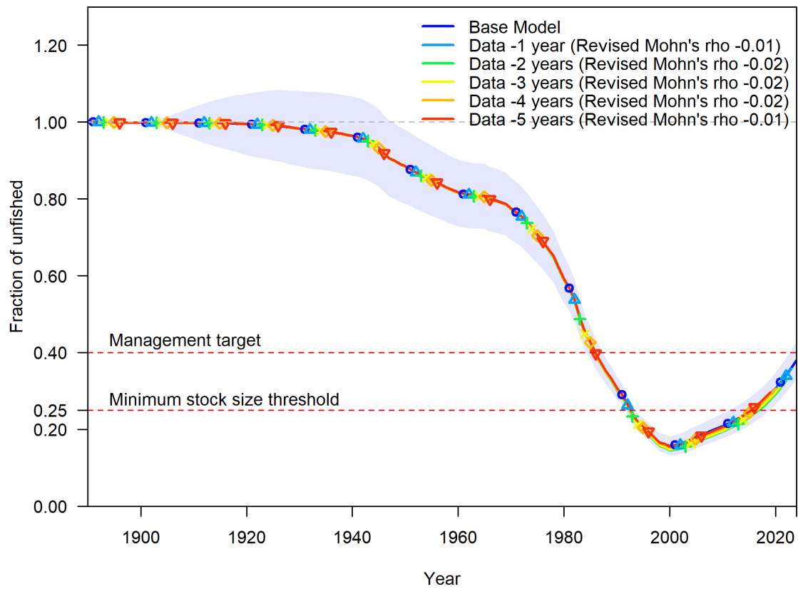
Figure 78: Results of retrospective analysis. Relative spawning output time series of this assesment base model are proved with \sim 95\% interval.
