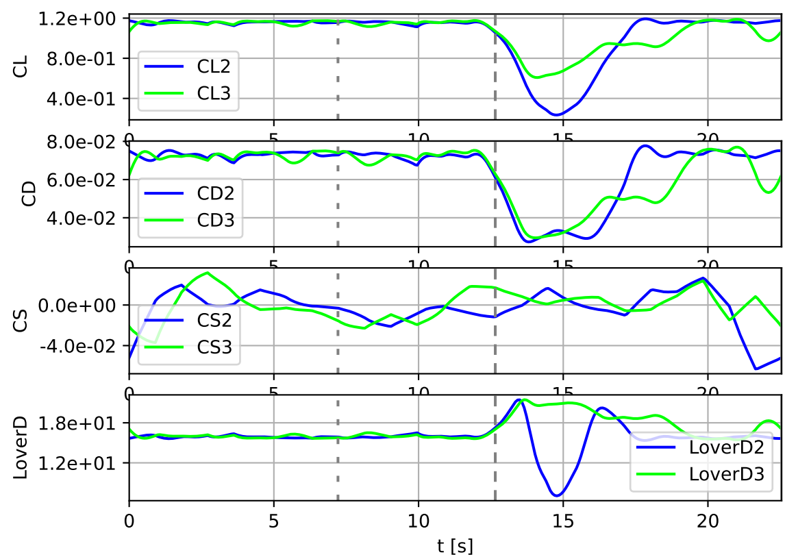
convergence_n_k_25_periods_tracked_2.8056471545263935_tol_1e-08_2026-01-08_8610324_aero_coefficients_plot
