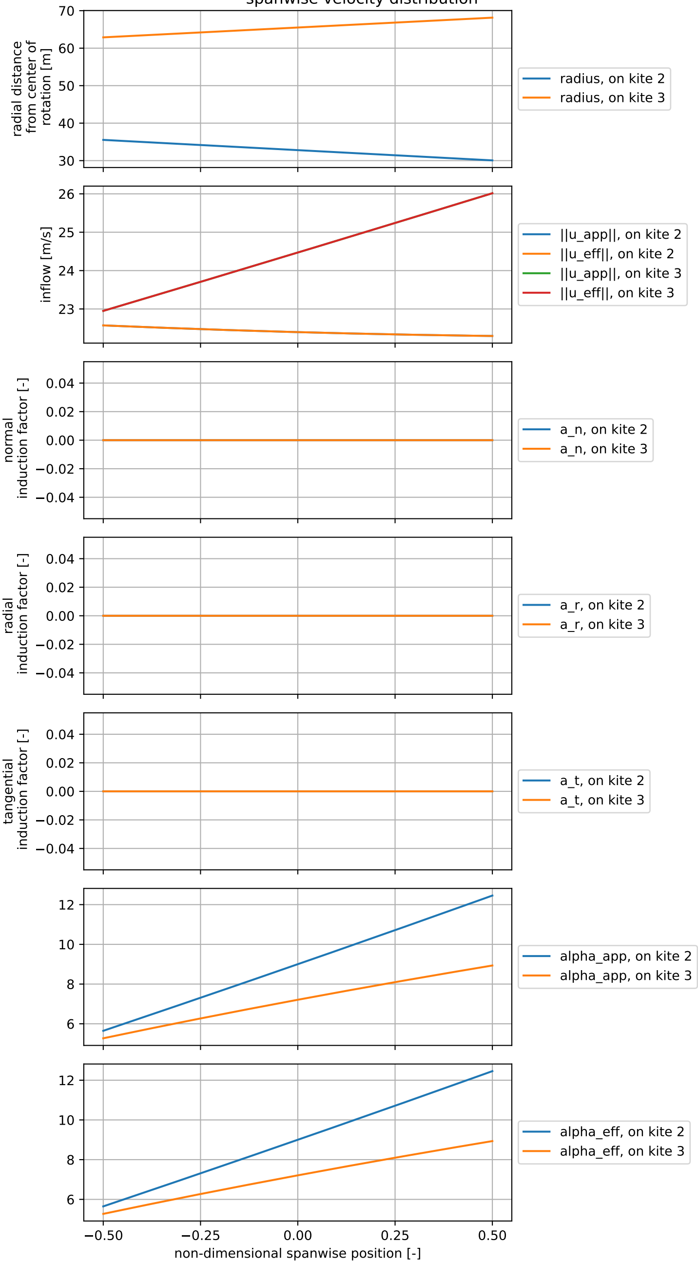
spanwise velocity distribution
