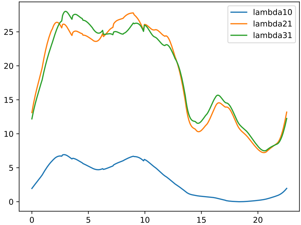
convergence_n_k_25_periods_tracked_2.8056471545263935_tol_1e-08_2026-01-08_8610324_algebraic_variables_plot
