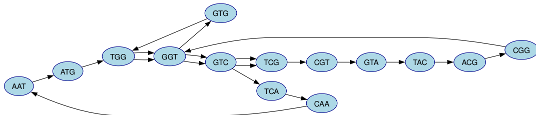
Figure 14: GGraph for kmers of size 4 for sequence TCGTACGGTCAATGGTGGTCG
