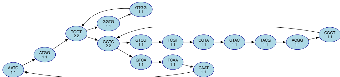
Figure 15: Graph for kmers of size 5 for sequence TCGTACGGTCAATGGTGGTTCG
