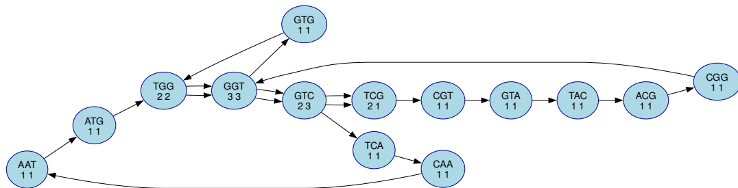
Figure 14: Graph for kmers of size 4 for sequence TCGTACGGTCAATGGTGGTTCG
