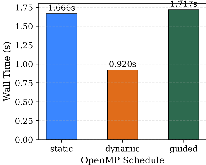
Wall Time by Schedule (N=2000, 8 threads, 500 steps)
