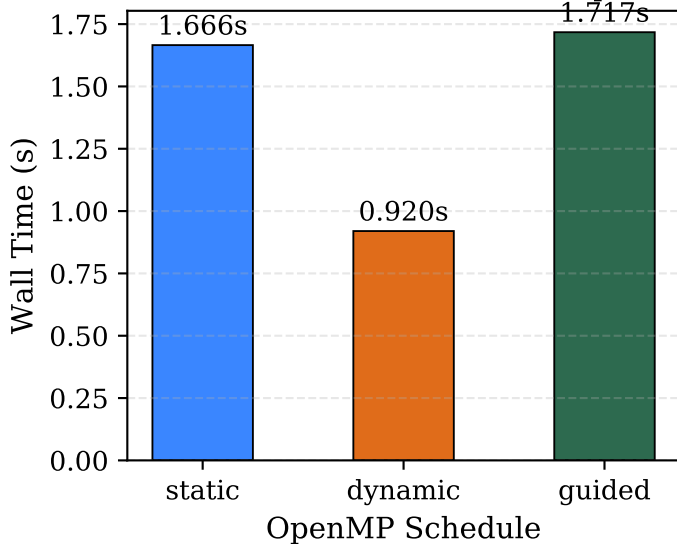
Wall Time by Schedule (N=2000, 8 threads, 500 steps)
