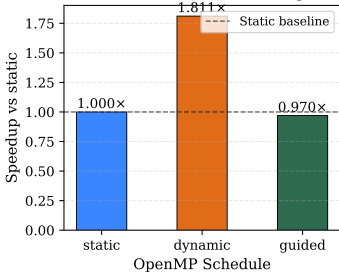
Relative Speedup vs Static (N=2000, 8 threads, 500 steps)
