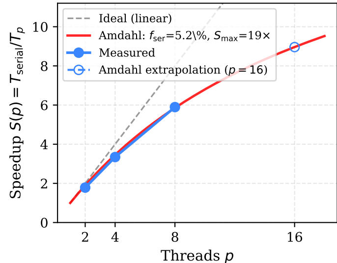
OpenMP Strong Scaling ( N = 2000 , 500 steps)
