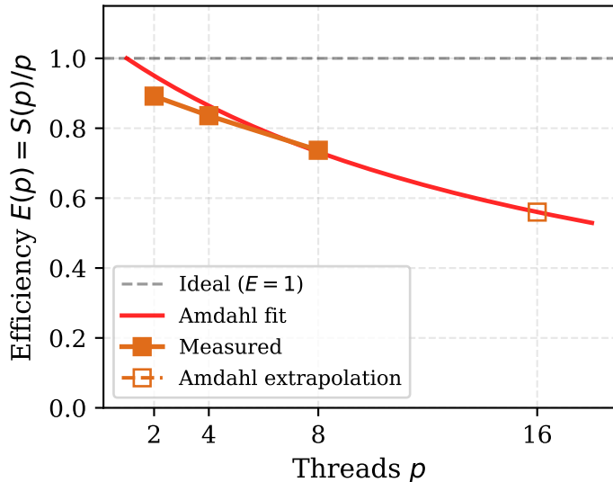
OpenMP Parallel Efficiency ( N = 2000 , 500 steps)
