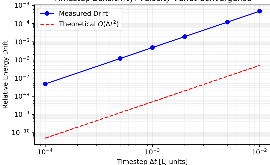
Timestep Sensitivity: Velocity Verlet Convergence
