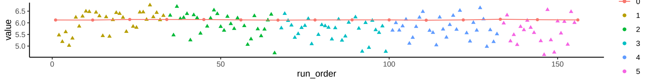
Compound: Ethanolamine
