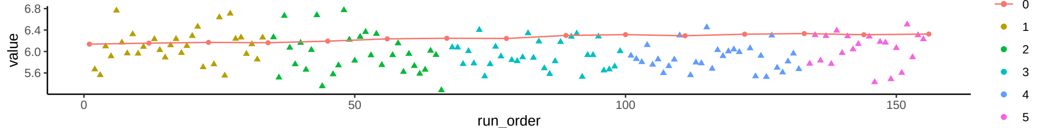
Compound: Arabitol/Xylitol
