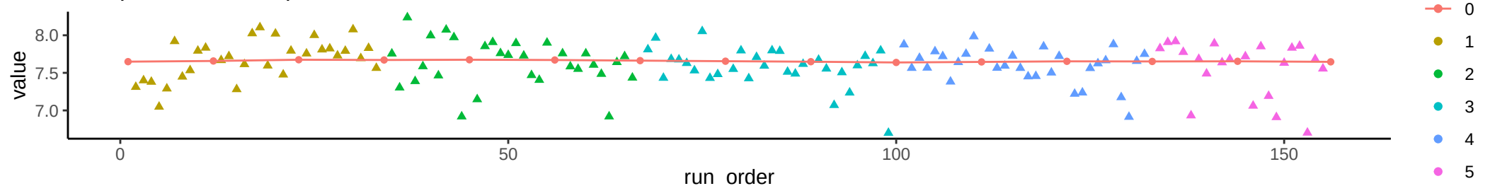
Compound: Ornithine
