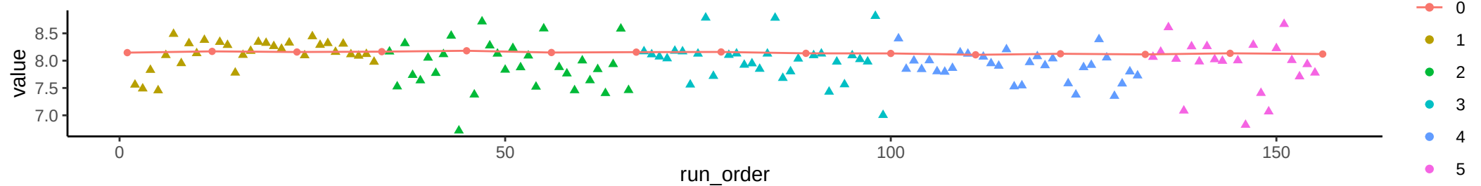
Compound: Glycine
