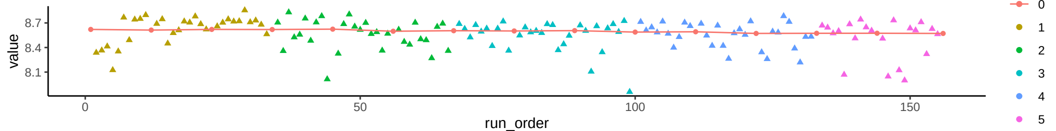
Compound: Arginine
