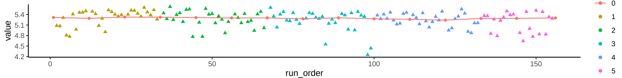
Compound: Agmatine
