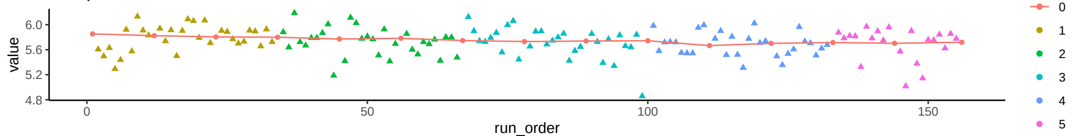
Compound: Orotate
