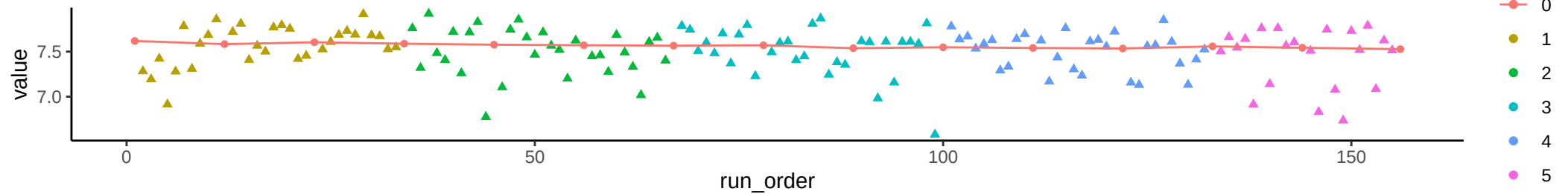
Compound: Carnitine
