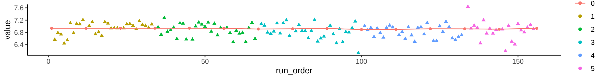
Compound: Lactose/Trehalose
