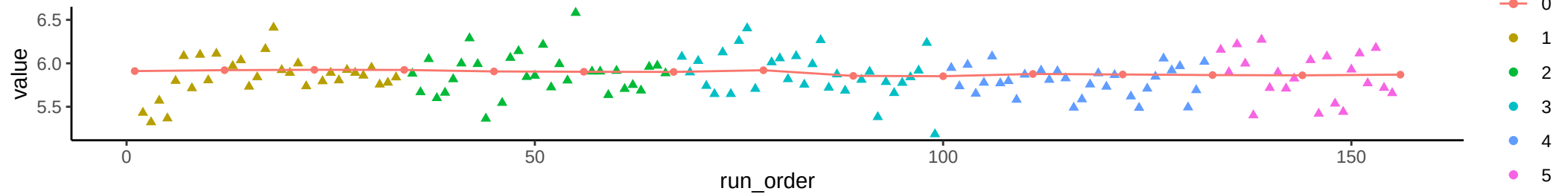
Compound: FAD
