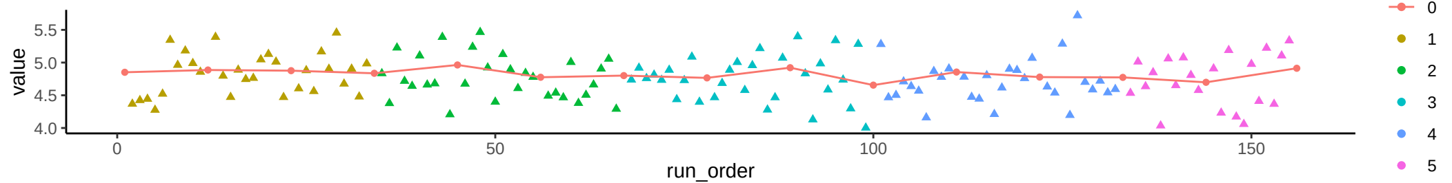
Compound: Deoxycarnitine
