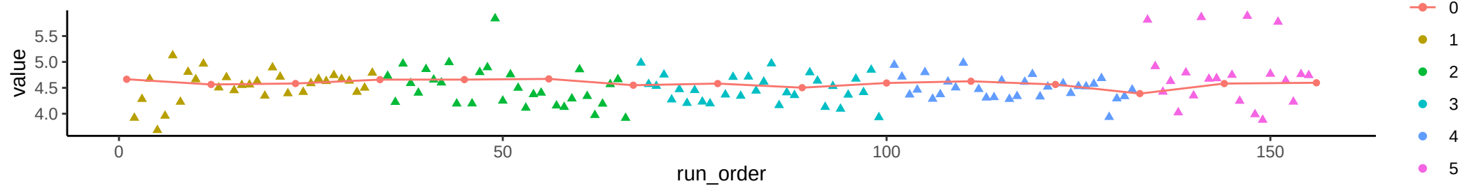
Compound: L-Kynurenine
