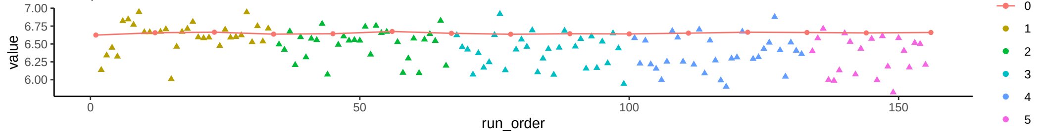
Compound: Adenosine
