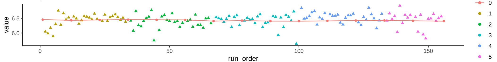
Compound: o-Phosphoethanolamine
