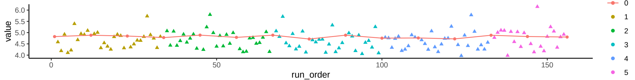
Compound: Lactate
