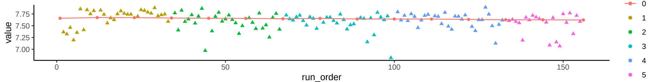
Compound: Allantoin
