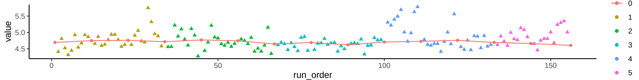
Compound: Adenine
