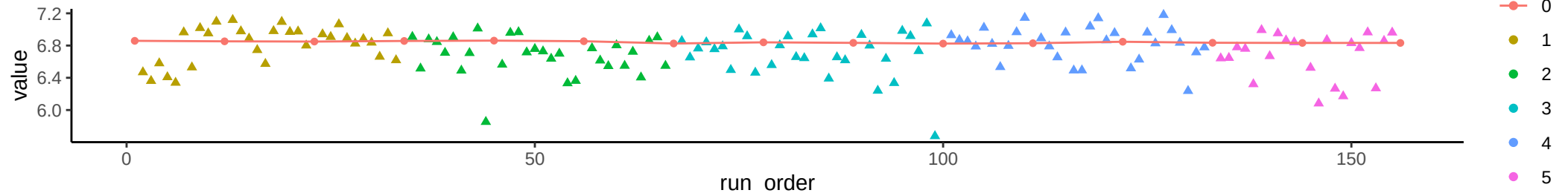
Compound: Arginine
