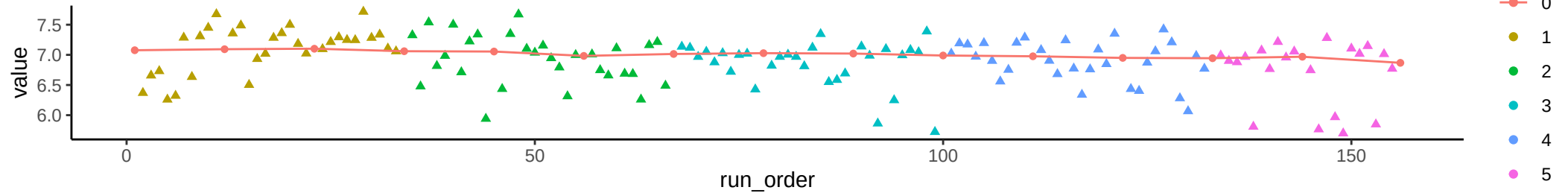
Compound: S-Methylcysteine
