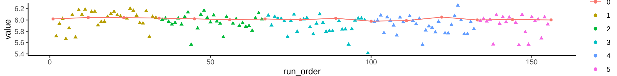
Compound: Fructose
