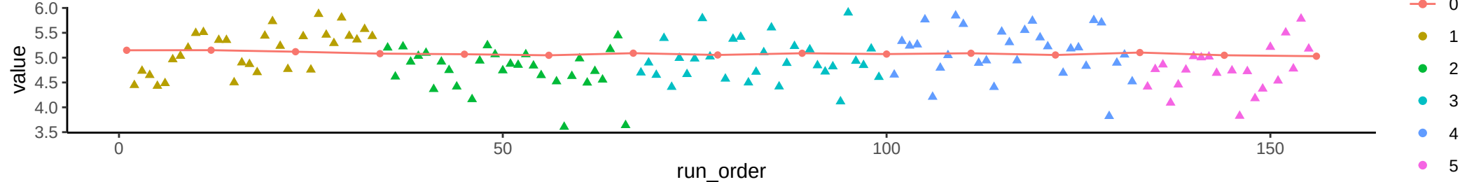
Compound: Carnitine
