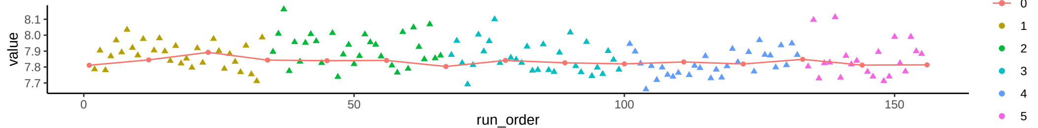
Compound: Biopterin
