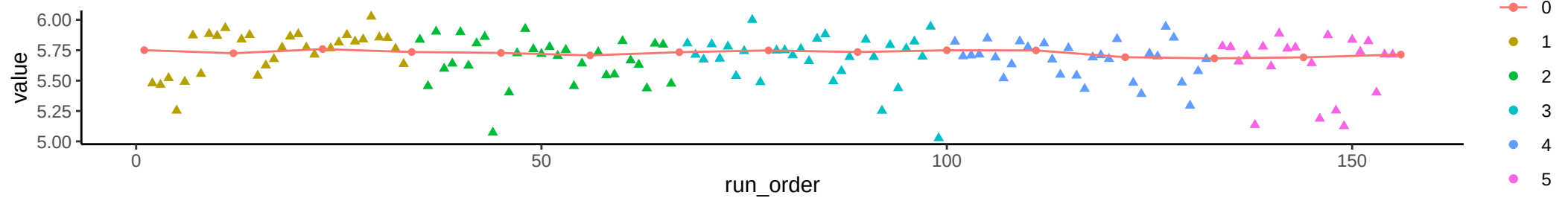
Compound: Alanine
