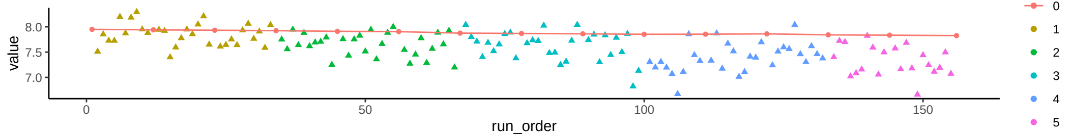
Compound: Adenylosuccinate
