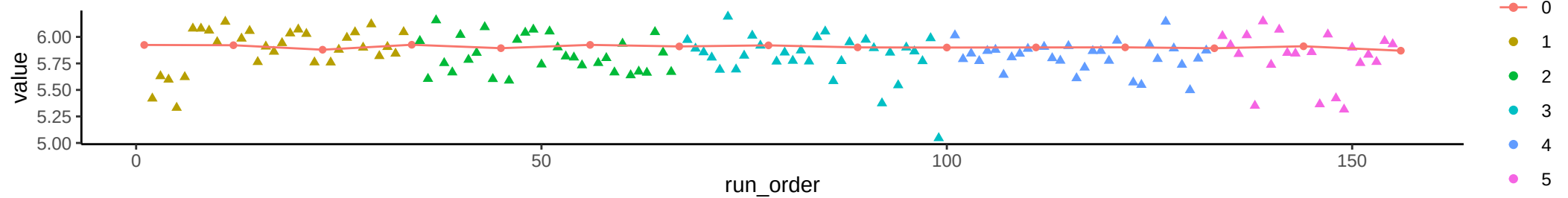
Compound: GMP
