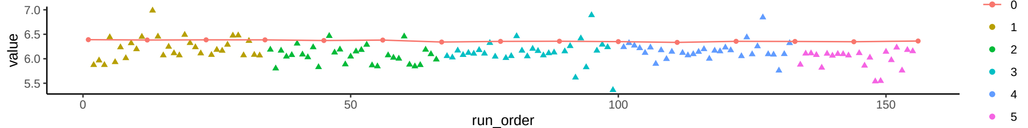
Compound: Putrescine
