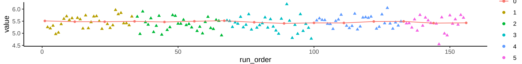
Compound: G1P/F1P/F6P
