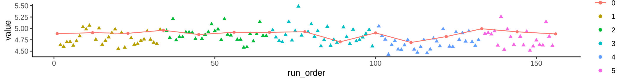
Compound: DCDP
