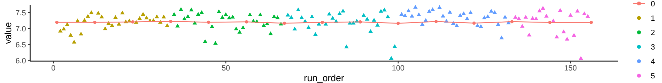
Compound: Guanine
