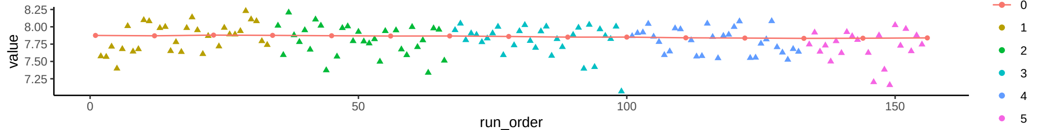
Compound: Pseudouridine
