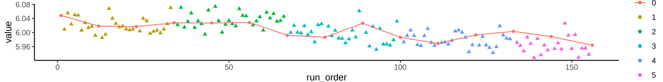
Compound: cAMP
