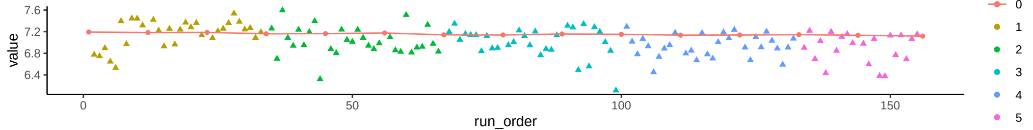
Compound: Guanosine
