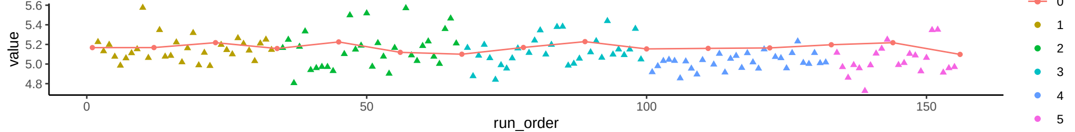
Compound: SAH
