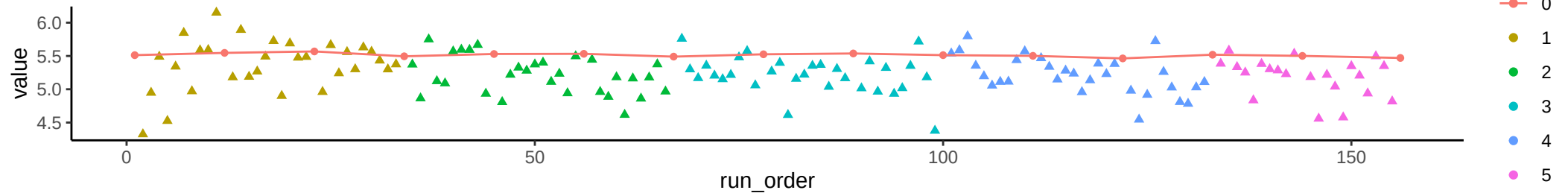
Compound: AMP
