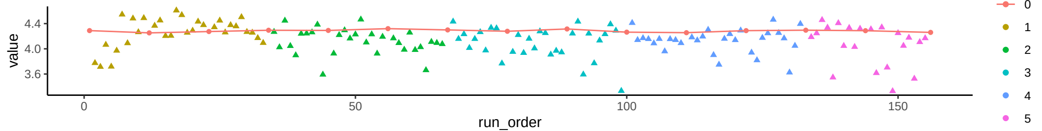
Compound: Deoxycarnitine
