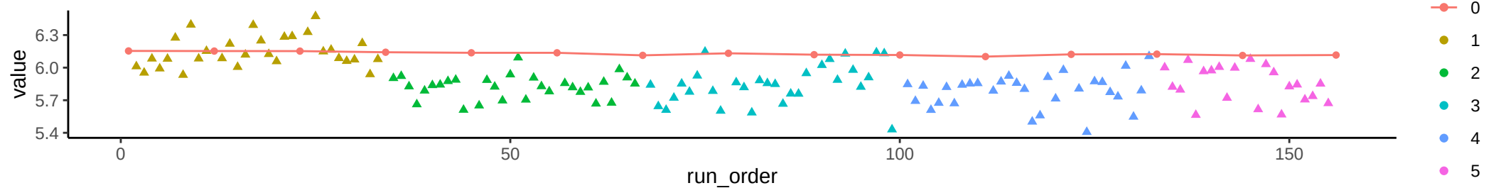
Compound: 3-Aminoisobutyrate
