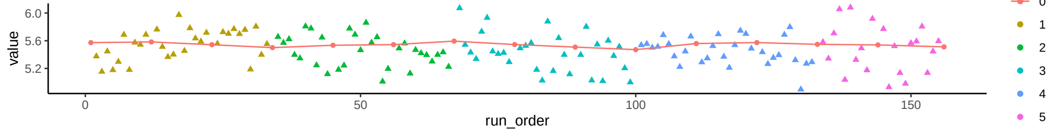
Compound: Proline
