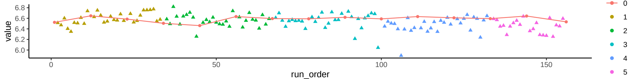
Compound: Pyridoxamine
