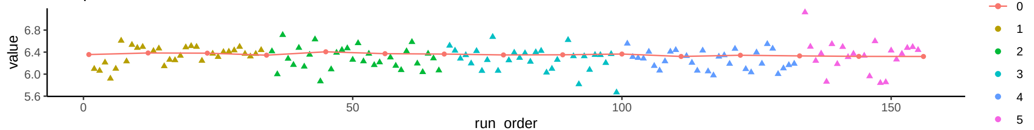
Compound: Orotate
