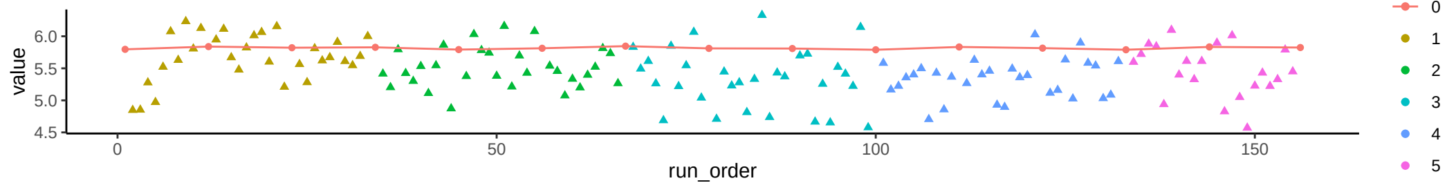
Compound: Cytidine
