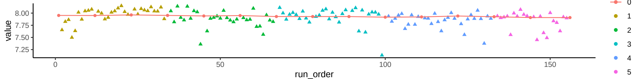
Compound: Cadaverine
