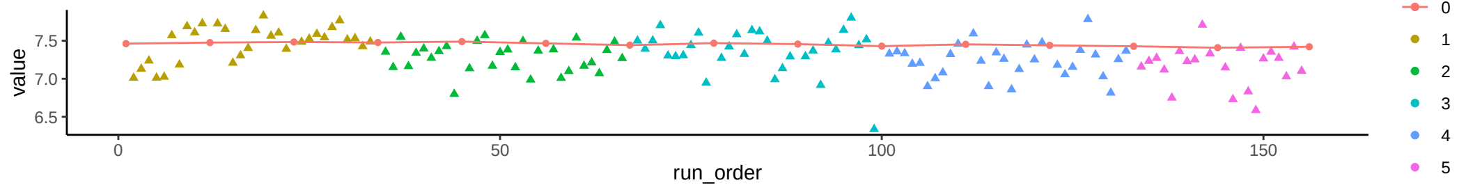
Compound: Guanosine
